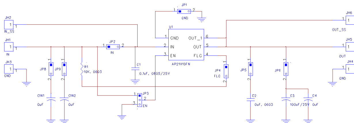
Figure 11. AP21X1AFM-EVM
