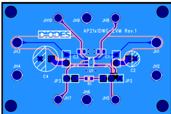
Figure 24. AP21X1AW-EVM – Top Layer
