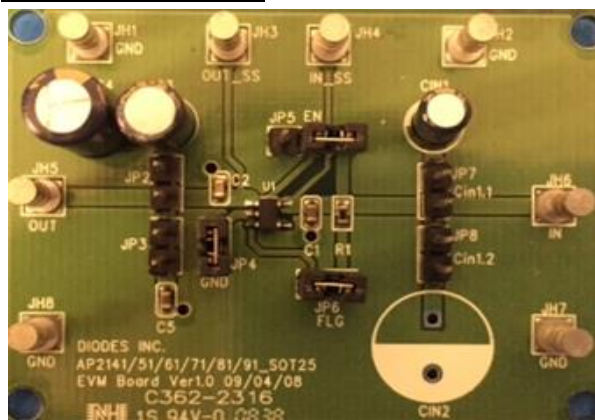
Figure 1. AP21X1AW-EVM
