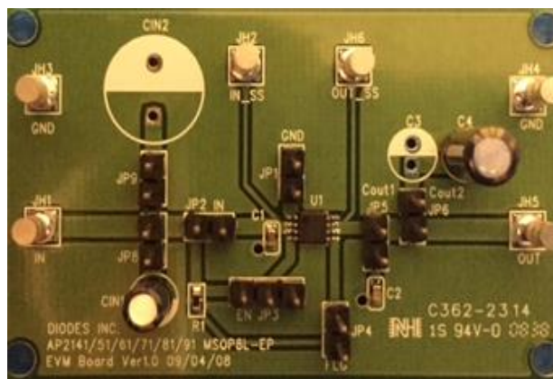
Figure 2. AP21X1AMP-EVM
