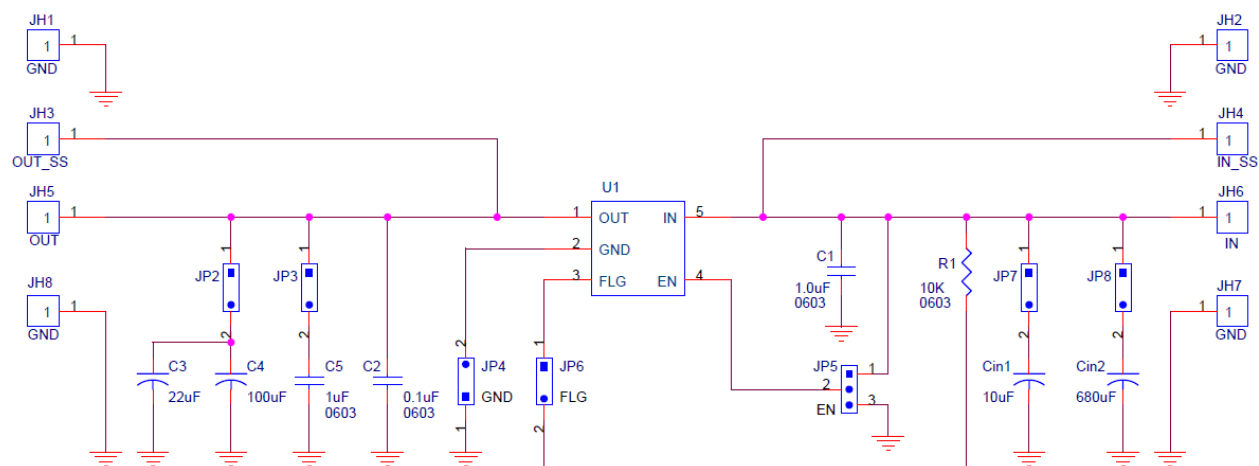
Figure 9. AP21X1AW-EVM
