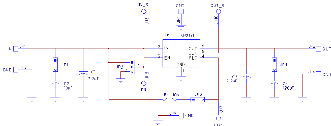
Figure 14. AP21X1AFM-EVM
