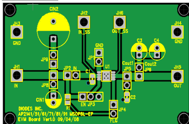
Figure 18. AP21X1AMP-EVM – Top Layer
