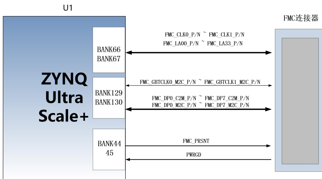
Figure 3-12-1: FMC Schematic
