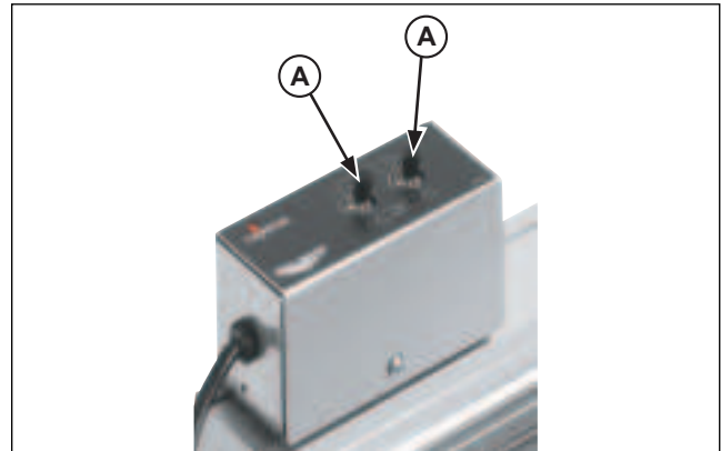
Figure 7. On Board Control with Switches
