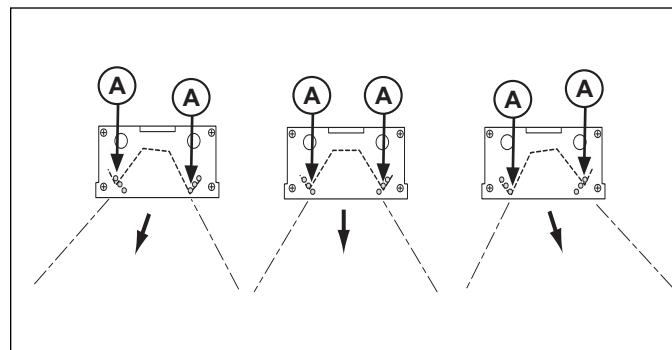
Figure 10. Reflector Positions.
