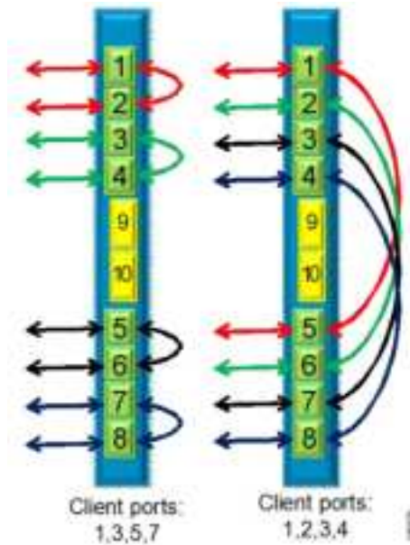
Figure 21: Low-Rate TXP_MR Card Operating Mode Configuration
