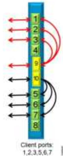
Figure 34: High-Rate MXP-VD-10G Card Operating Mode Configuration
