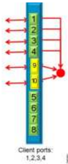
Figure 31: High-Rate MXPP-4x2.5-10G Card Operating Mode Configuration
