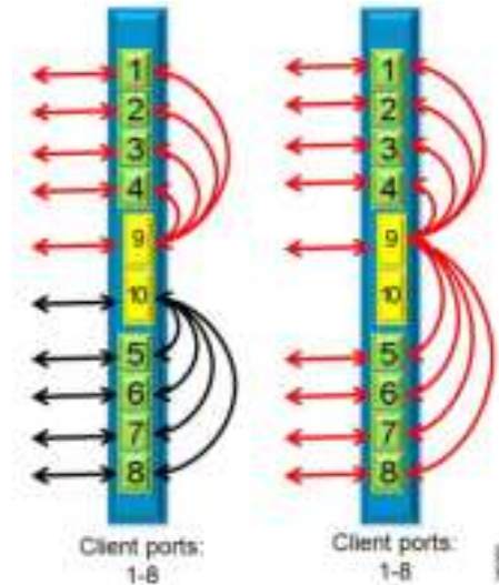
Figure 24: High-Rate MXP_DME Card Operating Mode Configuration
