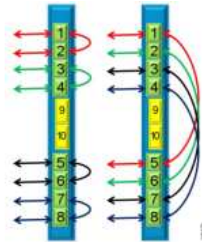
Figure 32: Low-Rate RGN Card Operating Mode Configuration
