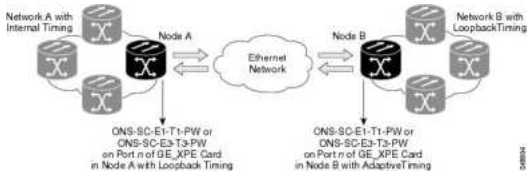
Figure 16: Recommended Topology for Using ONS-SC-E1-T1-PW and ONS-SC-E3-T3-PW SFPs
