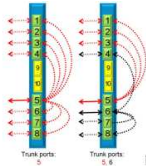
Figure 26: Low-Rate MXP_MR Card Operating Mode Configuration
