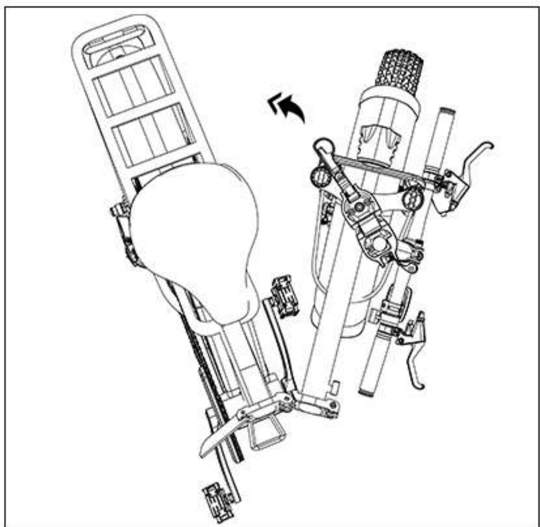
6. Release the kickstand. Grip the arc-shaped frame handle, and then slightly turn the front wheel to fold the mainframe.
