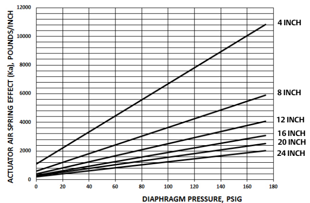
Figure 17. Size 280 Fisher 785C Double Acting Springless Actuator Spring Effect vs Diaphragm Pressure
