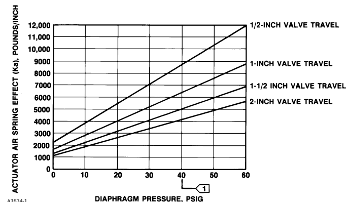
Figure 11. Size 46/46i or 60/60i Fisher 657, or Size 46/46i or 60 667 Actuator Air Spring Effect vs Diaphragm Pressure
