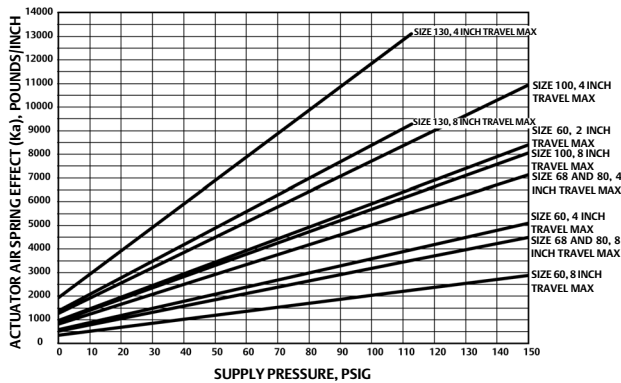
Figure 16. Size 60 through 130 Fisher 585C Actuator Air Spring Effect versus Supply Pressure
