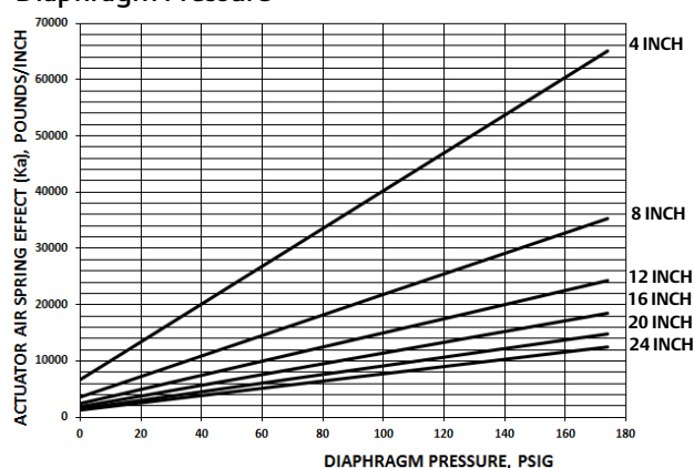
Figure 25. Size 685 Fisher 785C Double Acting Springless Actuator Spring Effect vs Diaphragm Pressure
