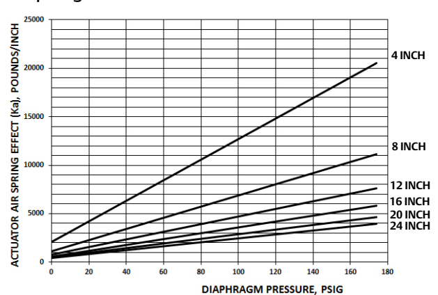
Figure 19. Size 385 Fisher 785C Double Acting Springless Actuator Spring Effect vs Diaphragm Pressure
