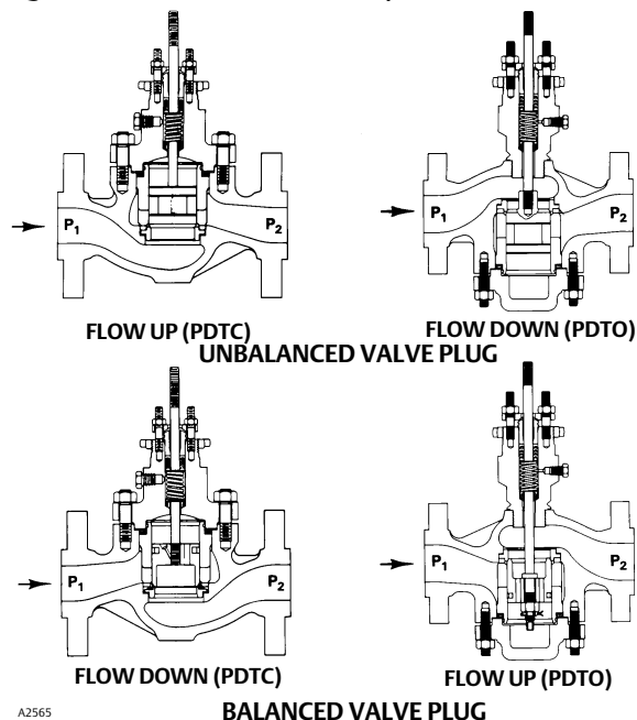
Figure 1. Pressure-Tends-To-Open
