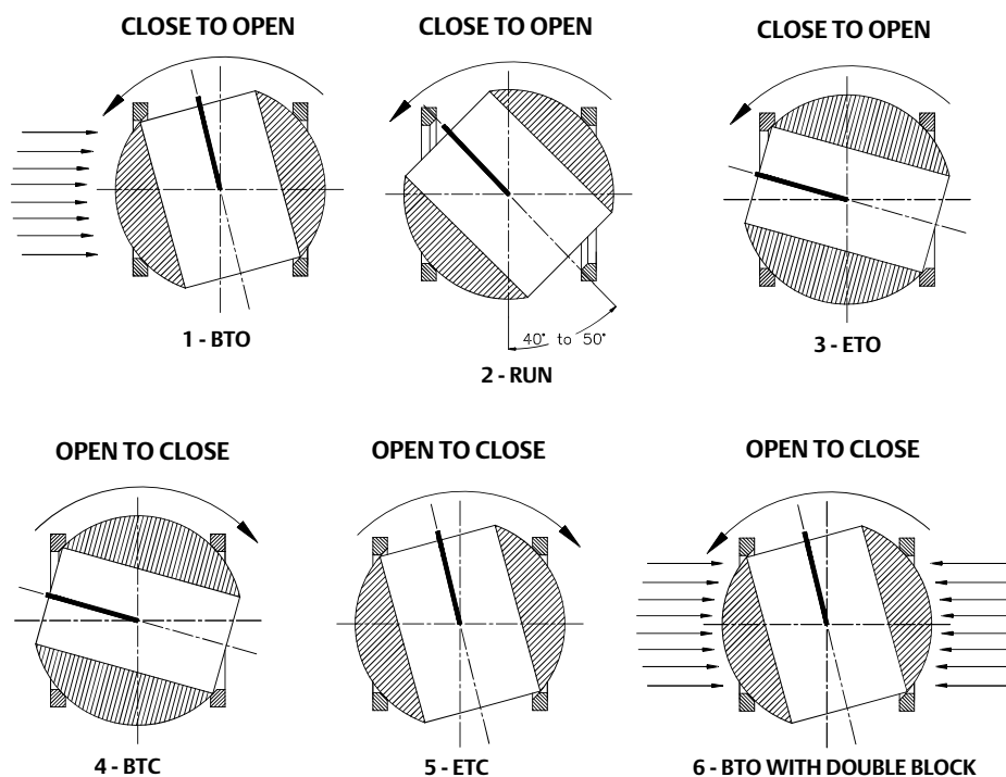
Figure 1. SIS Ball Valve Torque Terminology Ball Positions
