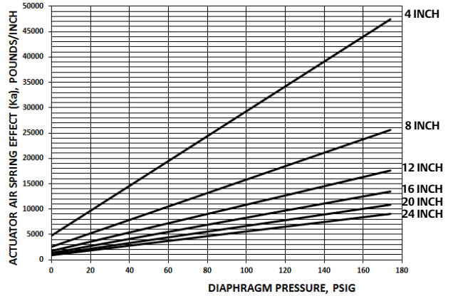
Figure 23. Size 585 Fisher 785C Double Acting Springless Actuator Spring Effect vs Diaphragm Pressure
