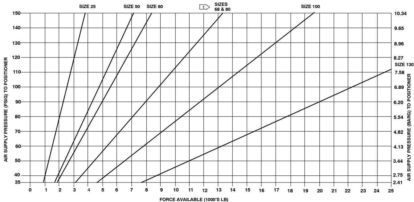
Figure 5. Fisher 585C Piston Actuator Force when used with 3600 Series Positioner or DVC6000 Digital Valve Controller
