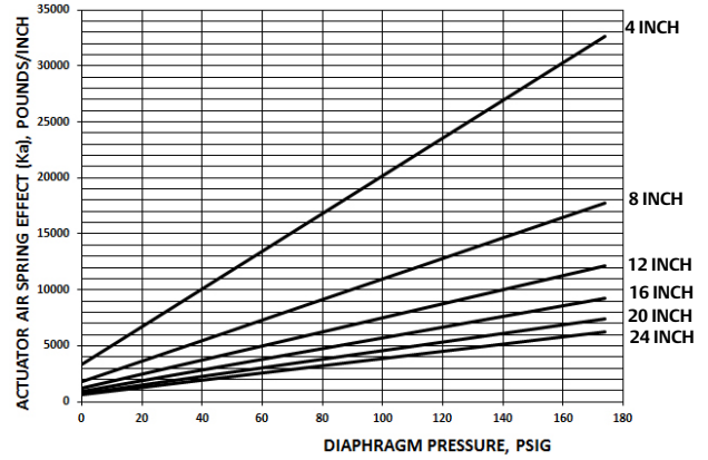
Figure 21. Size 485 Fisher 785C Double Acting Springless Actuator Spring Effect vs Diaphragm Pressure
