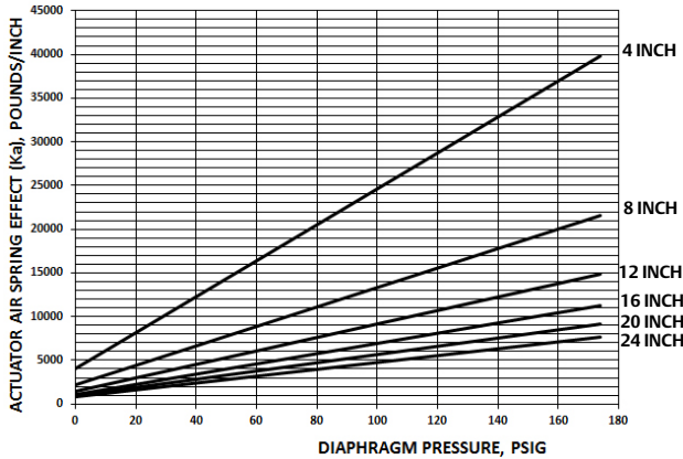
Figure 22. Size 535 Fisher 785C Double Acting Springless Actuator Spring Effect vs Diaphragm Pressure
