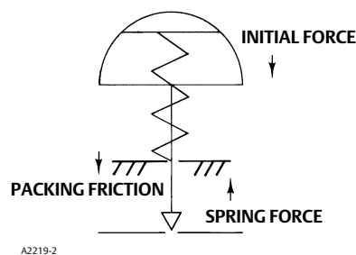
Figure 26. Fisher 657 Actuator Free Body Diagram
