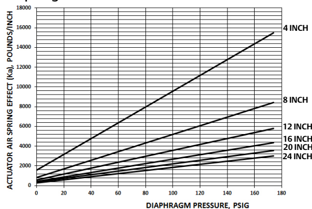
Figure 18. Size 335 Fisher 785C Double Acting Springless Actuator Spring Effect vs Diaphragm Pressure
