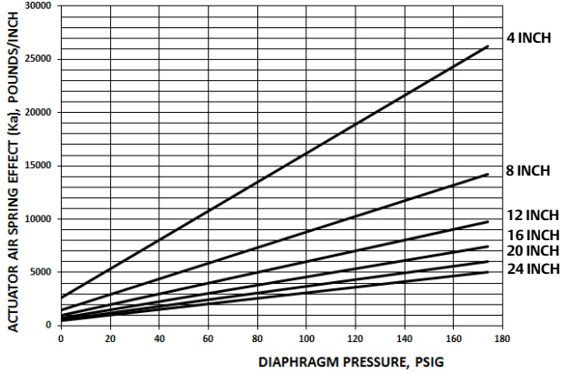
Figure 20. Size 435 Fisher 785C Double Acting Springless Actuator Spring Effect vs Diaphragm Pressure
