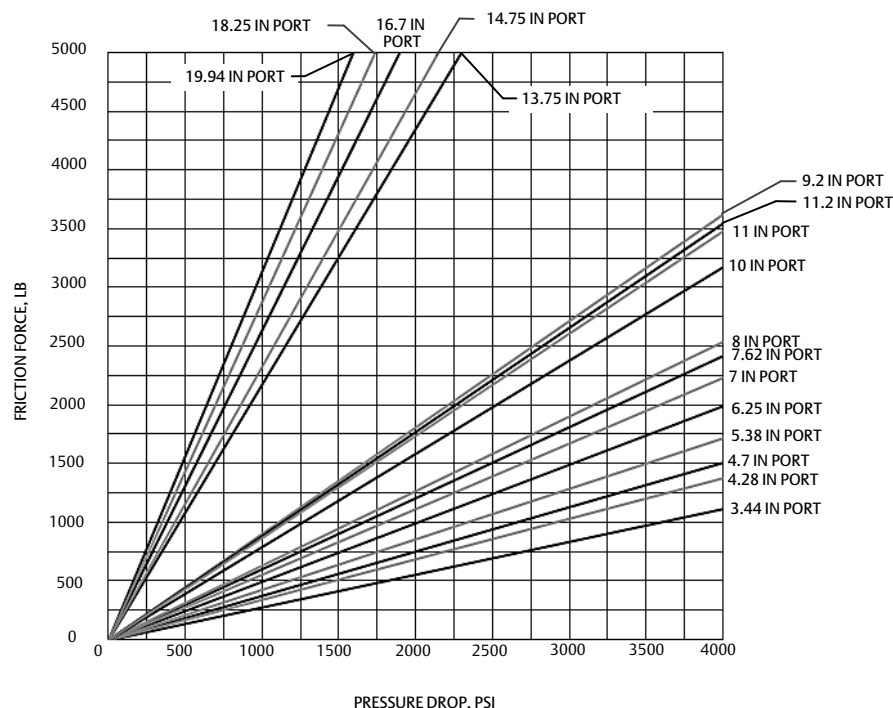
Figure 4A. Fisher TBX & CVX Metal Piston Ring Friction Forces
