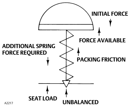
Figure 27. Fisher 667 Actuator Free Body Diagram
