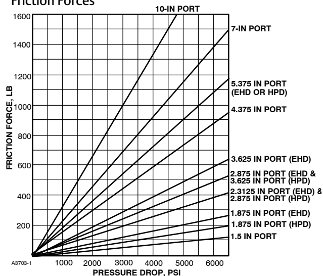
Figure 4. Fisher EHD & HPD Graphite Piston Ring Friction Forces
