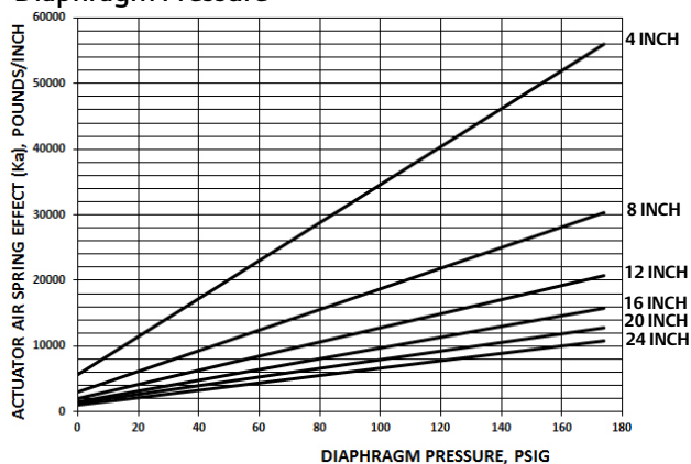
Figure 24. Size 635 Fisher 785C Double Acting Springless Actuator Spring Effect vs Diaphragm Pressure
