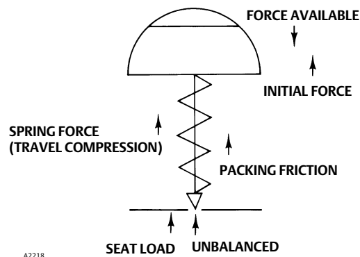
Figure 6. 657 Actuator Free Body Diagram
