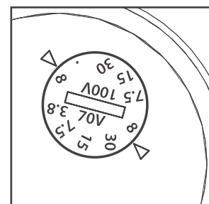
FIGURE 15: TRANSFORMER TAP SELECTOR
