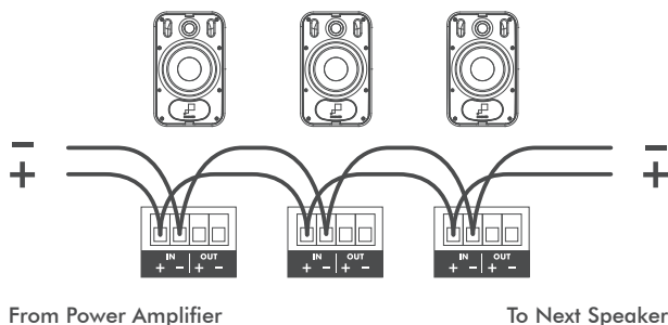
FIGURE 13: PARALLEL CONNECTION
