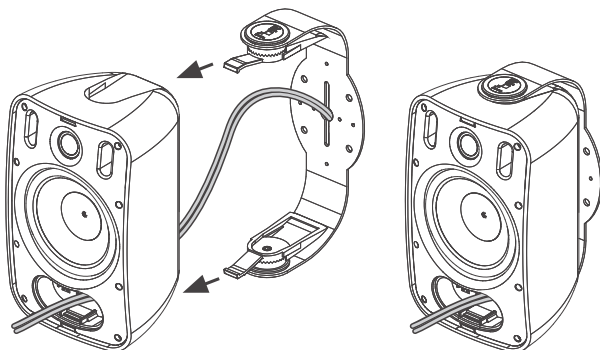
FIGURE 10: ATTACH SPEAKERS TO BRACKETS
