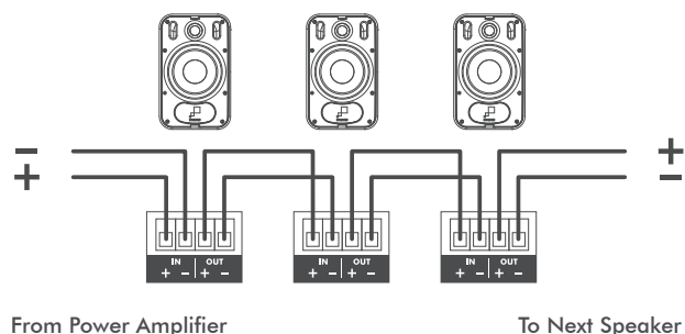
FIGURE 14: LOOP THRU CONNECTION
