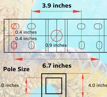
C-b. STLSTC-TRS-20W/30W (for SUNLIKE 20W/30W) works with 2.0 inches to 4.0 inches poles.
