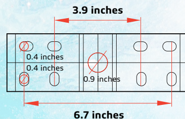
A-b. STLSTC-WM-20W/30W (for SUNLIKE 20W/30W)
