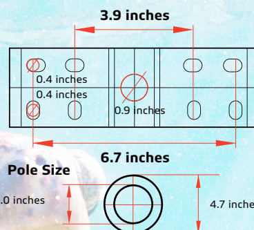
B-b. STLSTC-TRR-20W/30W (for SUNLIKE 20W/30W) works with 2.0 inches to 4.7 inches poles.
