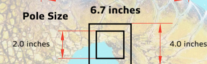
C-b. STLSTC-TRS-20W/30W (for SUNLIKE 20W/30W) works with 2.0 inches to 4.0 inches poles.
