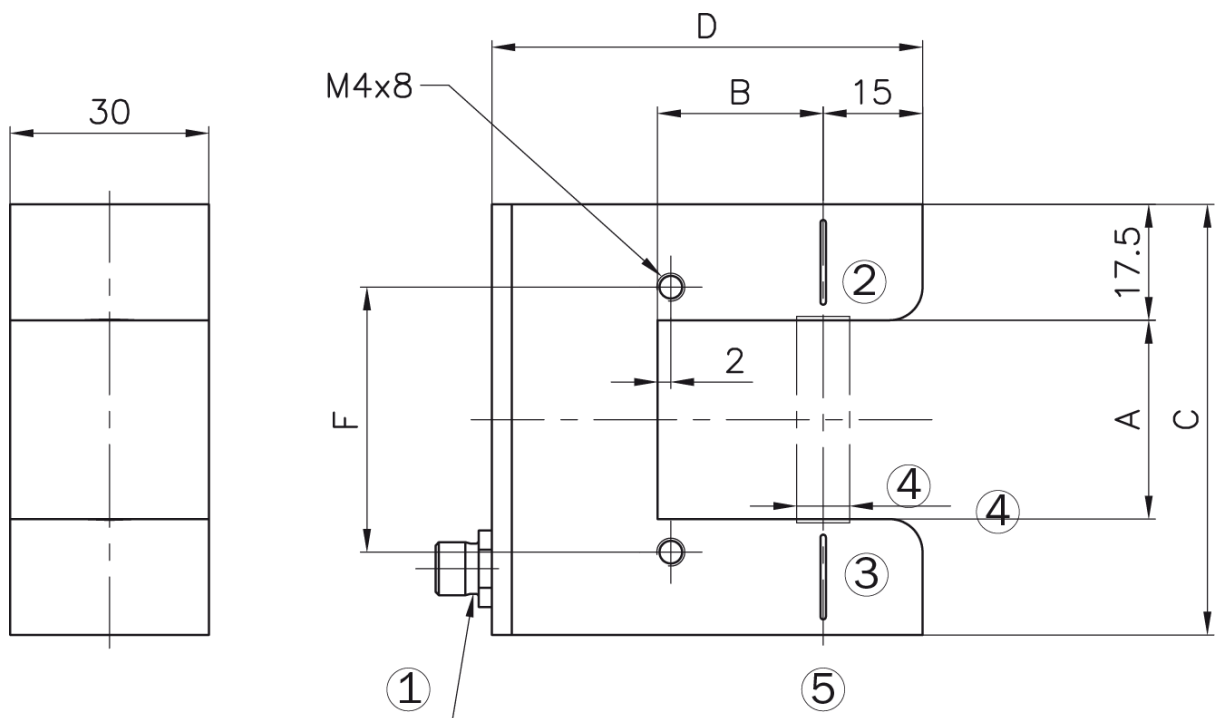
Figure 1: Dimensions US01_04B.ai
