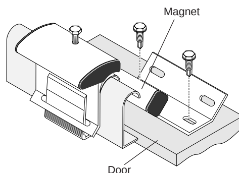
Figure 2 - Attaching Magnet to Door
