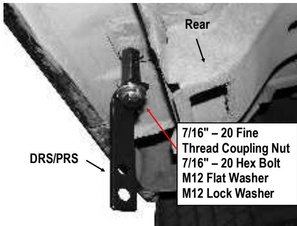
(Fig 8) Passenger Rear Support Bracket Installation
