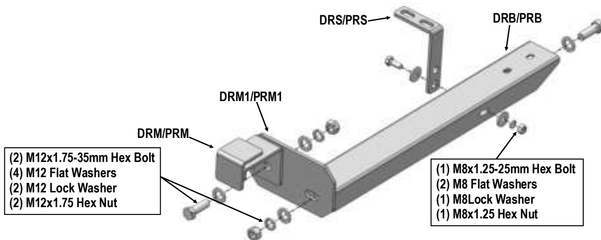
(Fig 9) Passenger Side Rear Brackets Assembly
