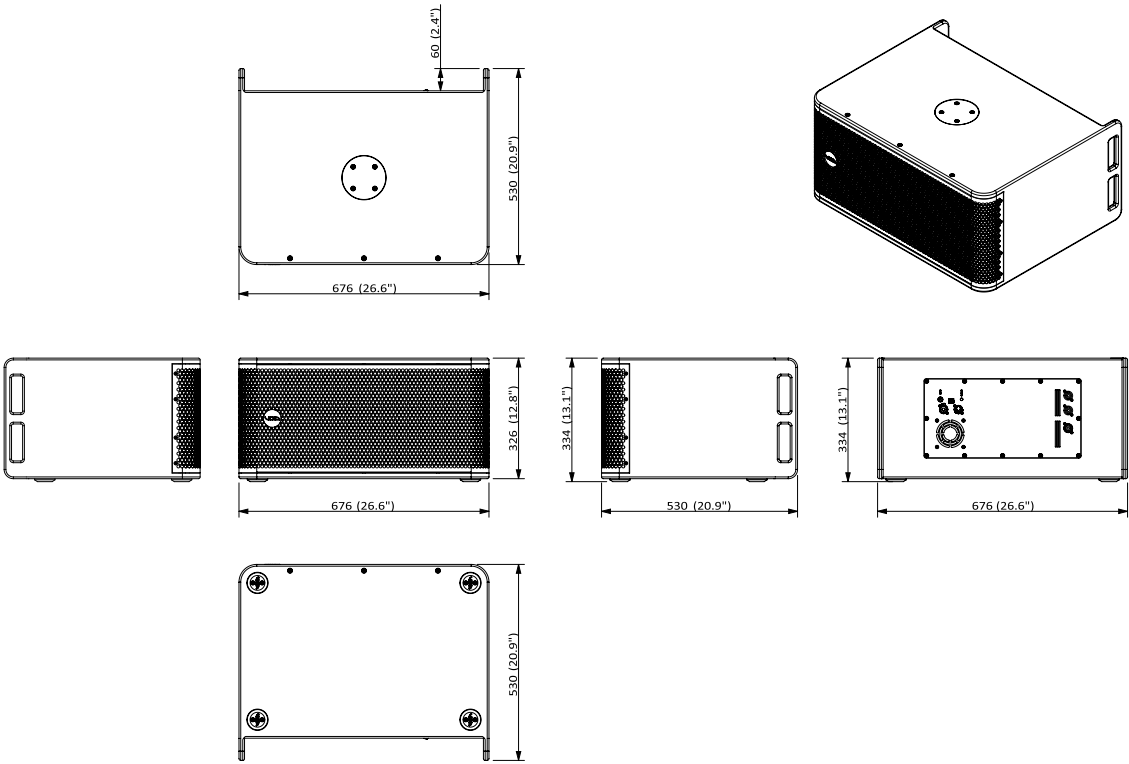
Figure 3.1: Dimensions
