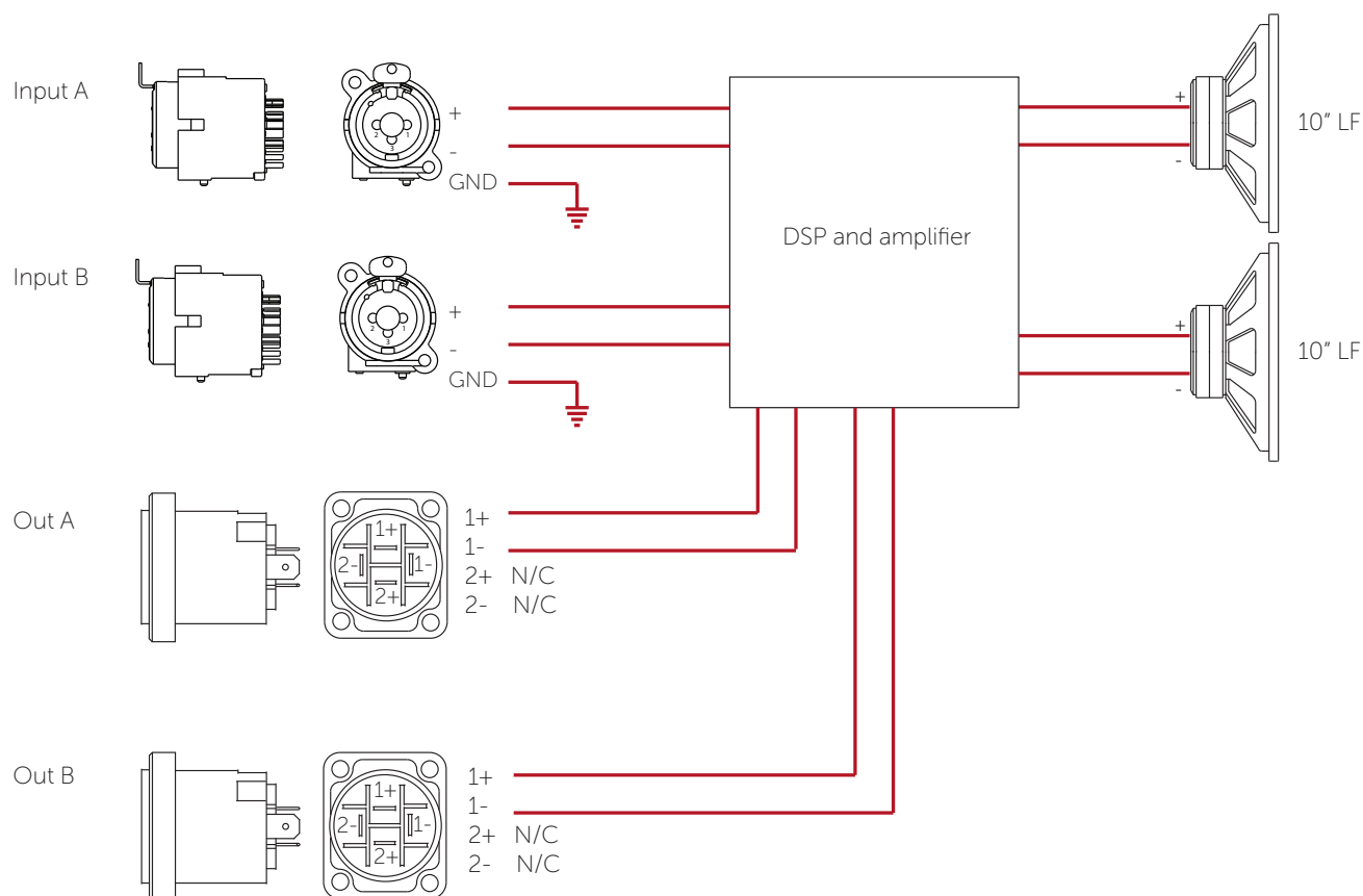
Figure 4.1: Venu 210i V2 wiring diagram
