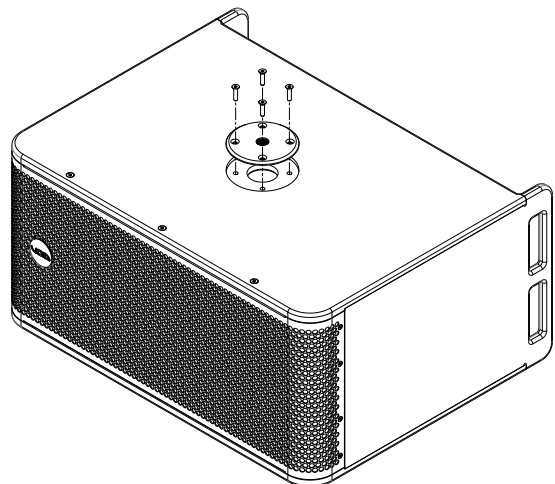
Figure 6.3: Top hat placement
