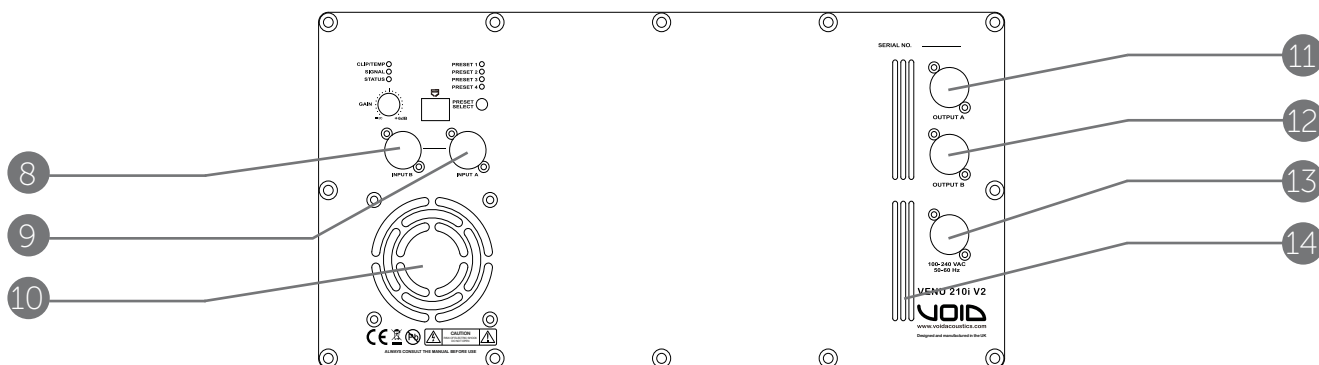
Figure 5.2: Rear panel
