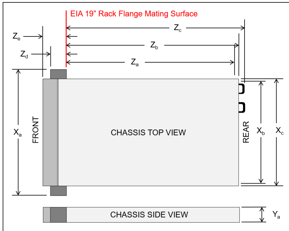
Figure 19. Server dimensions
