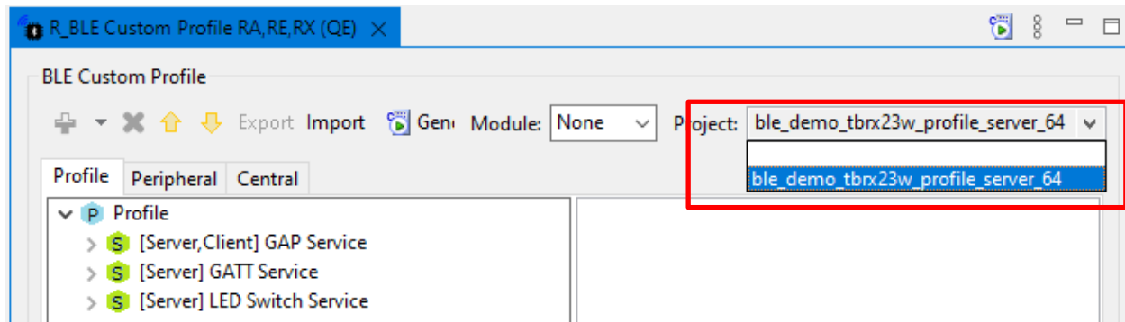
Figure 3.3 Select project
