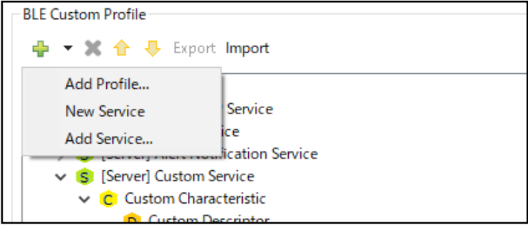
Figure 3.7 Adding service
