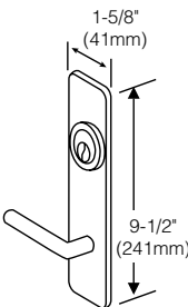
500F Series
