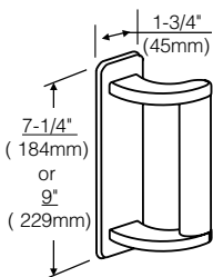
480F Series
