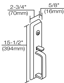
630F/660F Series
