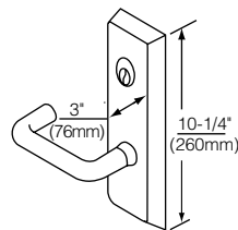
620F/650F Series
