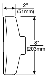
Cover Detail
