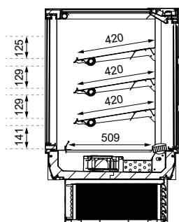
SECTION VIEW
