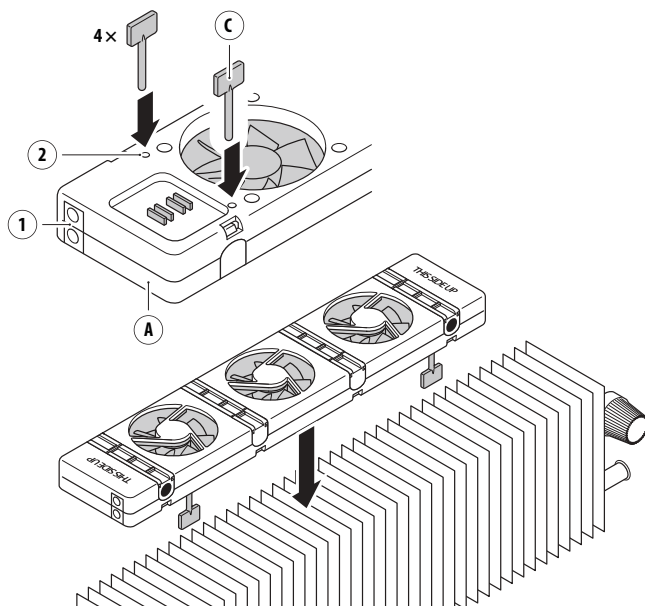
Fig. 8 - Attach a foot (C).
