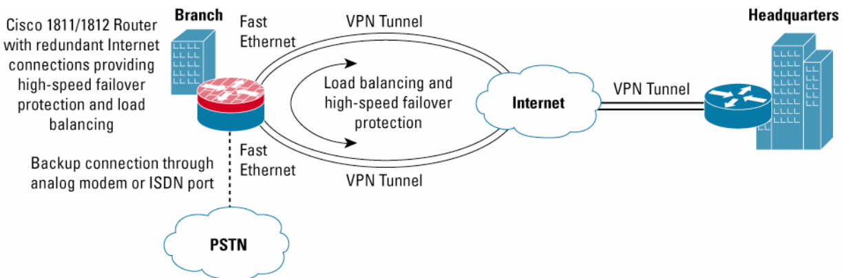
Figure 3. High-Availability Small Branch Network with Cisco 1811 or 1812 Router
