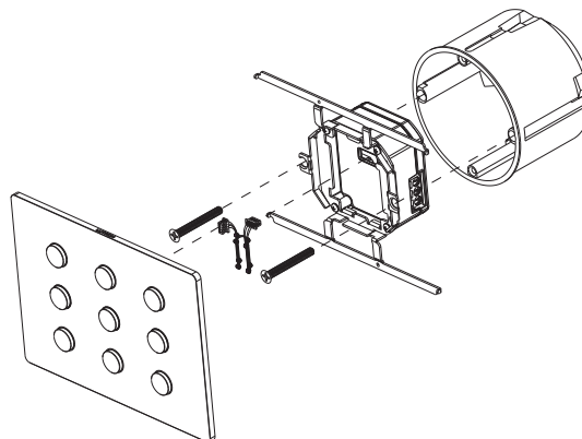
Three column 1,2,3
