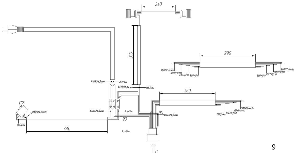
E-14 Led/Sliding control wiring diagram
