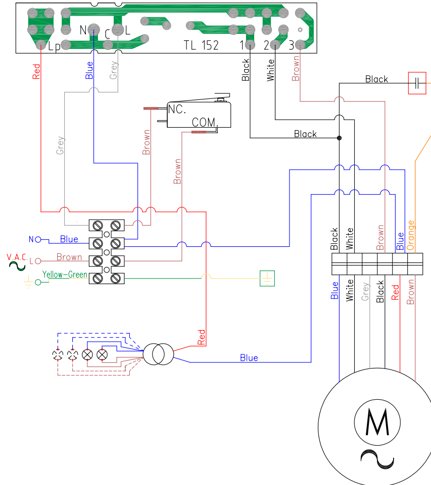
E-14 Led/Sliding control wiring diagram
