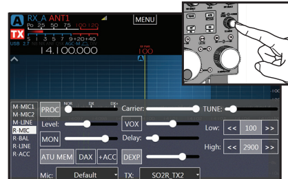
Press Power Knob for Transmit Menu
