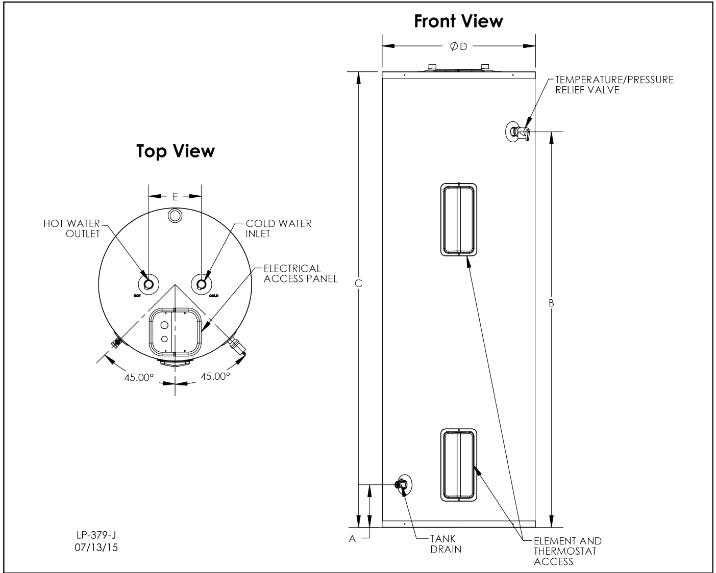
Figure 2 - Dimensional Drawing - Staged Operation
