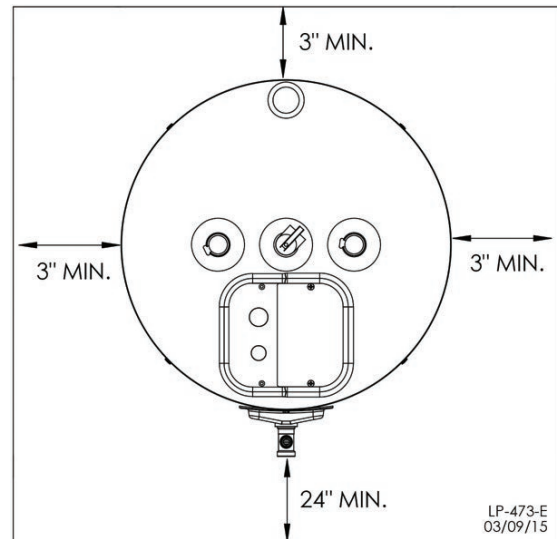
Figure 1 - Recommended Service Clearances - NOTE: Overhead View Not Representative of All Models
