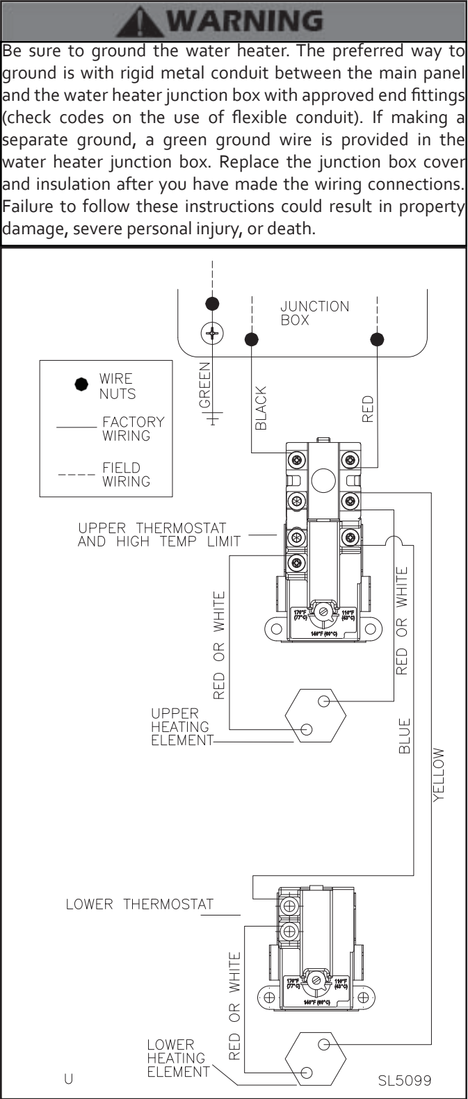
Figure 6 - Dual Element Model Wiring Detail, Staged Element Operation - Green Wire for Grounding the Water Heater - U Models
