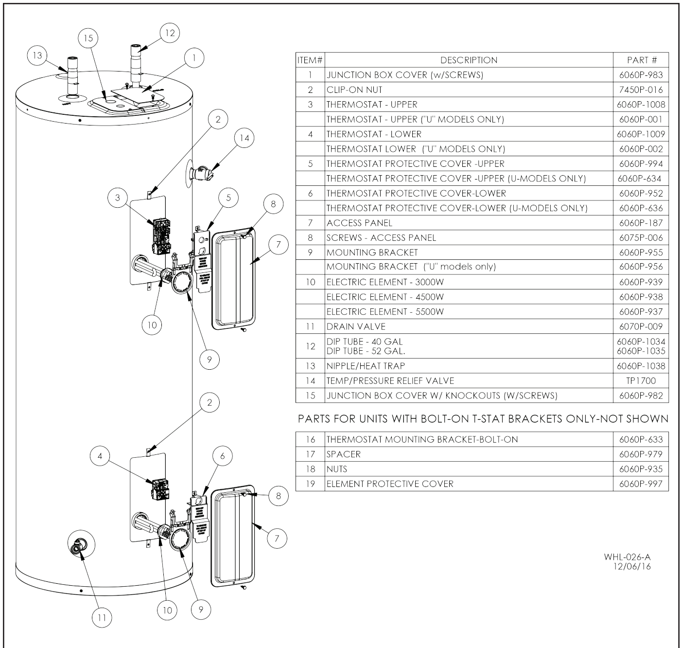
Figure 9 - Replacement Parts - Staged Operation
