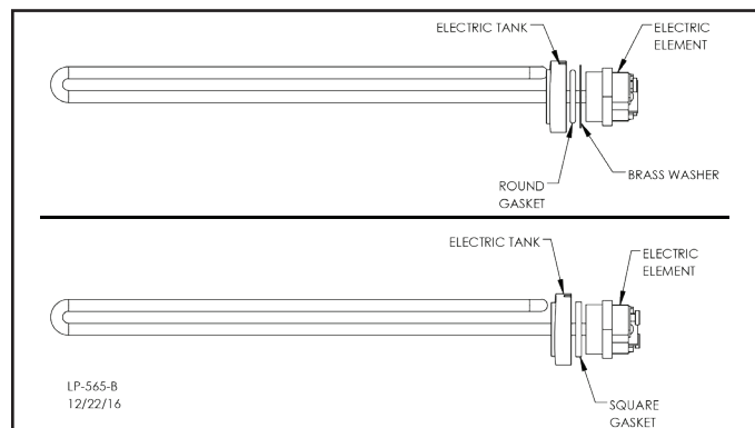
Figure 7 - Heating Element Detail
