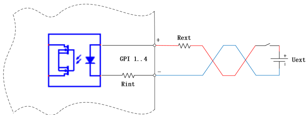
Fig.4-1: Internal and possible external wiring of the optocoupler inputs
