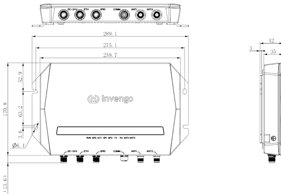
Fig. 3-1: Installation Drawing
