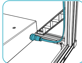
F. Connect the hotbed cable
