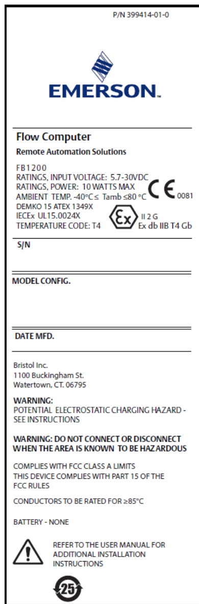
Figure 1. Emerson FB1200 Label (Flameproof)
