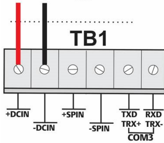
Figure 9. Wiring to DC Power Supply (without Optional I/O)
