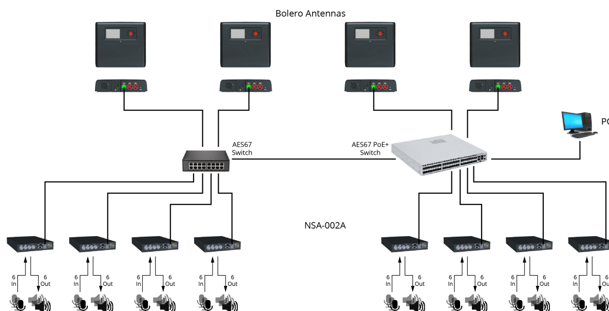
Figure 107: IO devices – setup diagram – Standalone/AES67 mode
