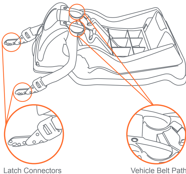
Latch Connectors
