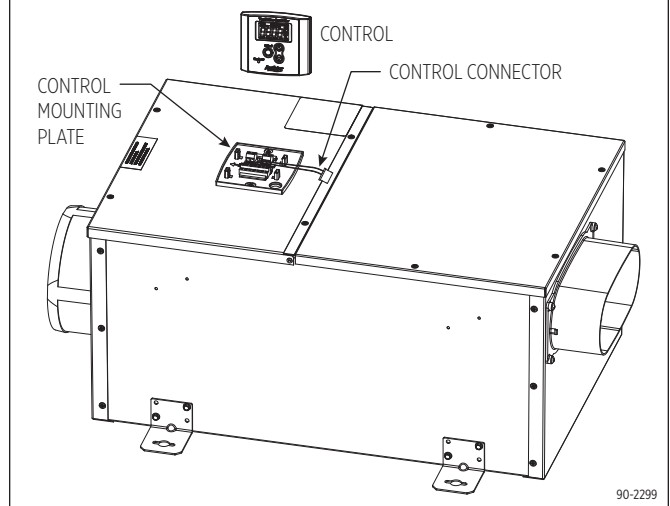
FIGURE 9 – REMOVE CONTROL FROM MOUNTING PLATE
