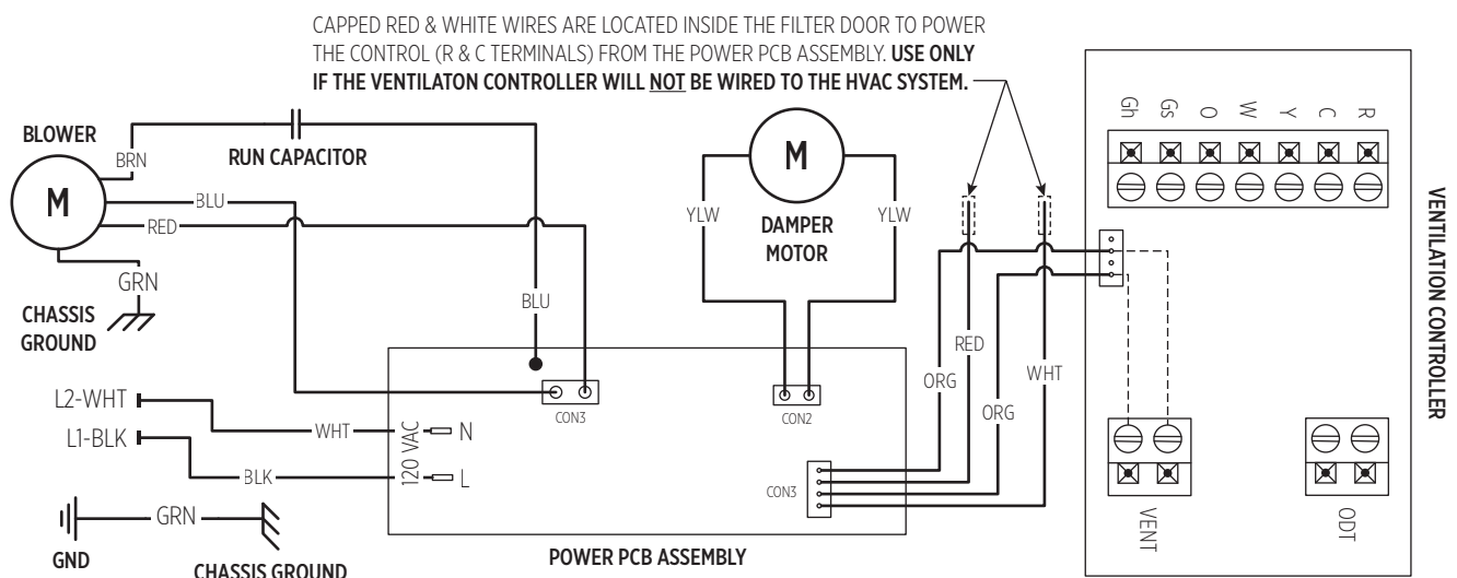
FIGURE 16 – MODEL 8140 INTERNAL SCHEMATIC
