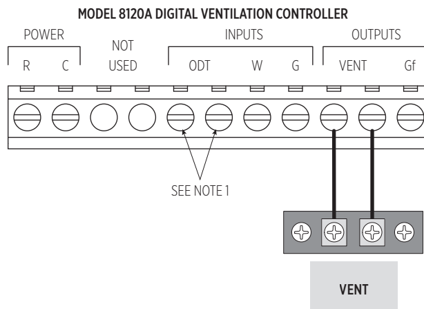
FIGURE 7 – WIRING TO MODEL 8120A
