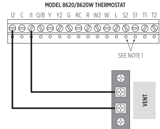
FIGURE 6 – WIRING TO THERMOSTAT
