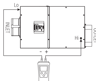
FIGURE 13 – MEASURE PRESSURE AT INLET AND OUTLET PRESSURE PORTS
