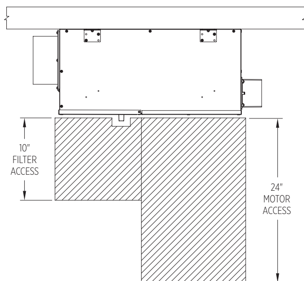
FIGURE 2 – CLEARANCES FOR SERVICING
