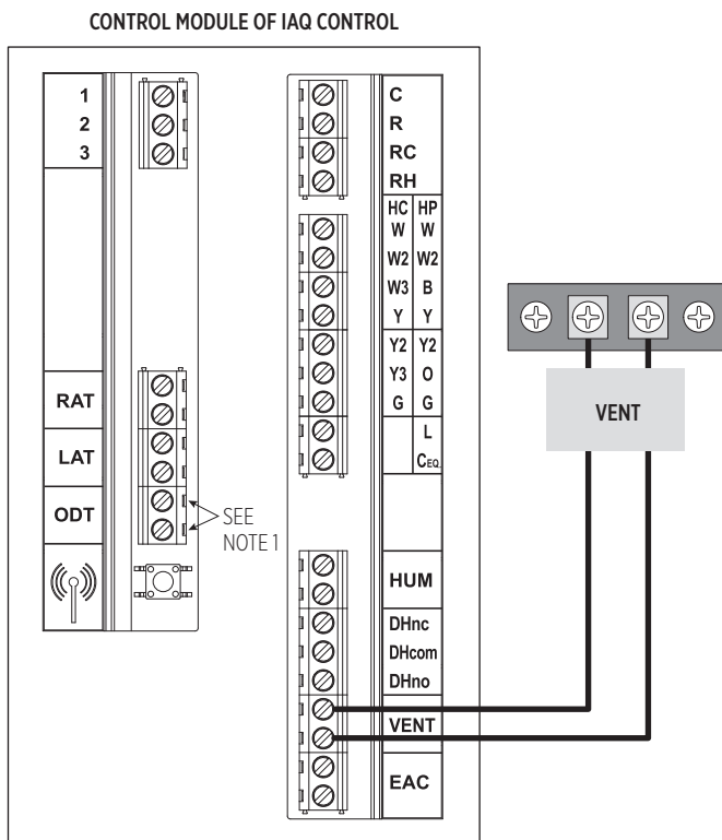
FIGURE 5 – WIRING TO IAQ CONTROL
