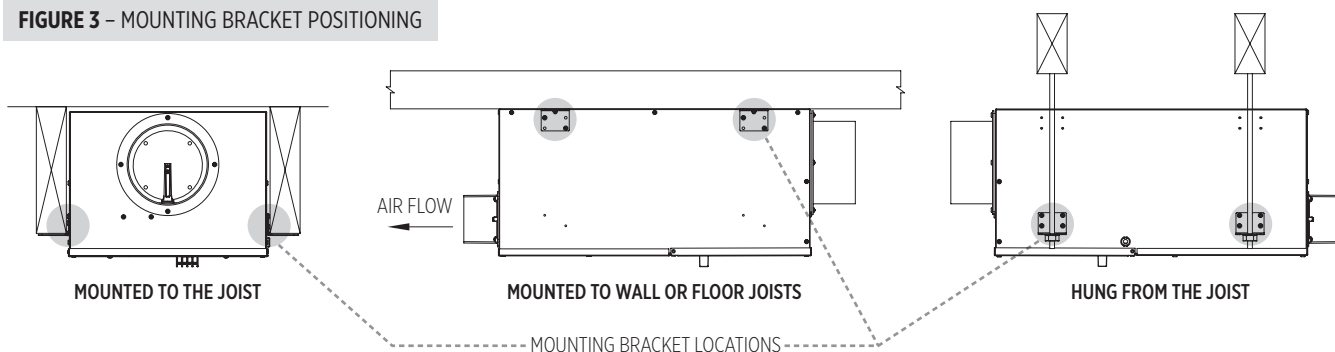
FIGURE 3 – MOUNTING BRACKET POSITIONING
