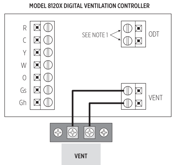
FIGURE 8 – WIRING TO MODEL 8120X
