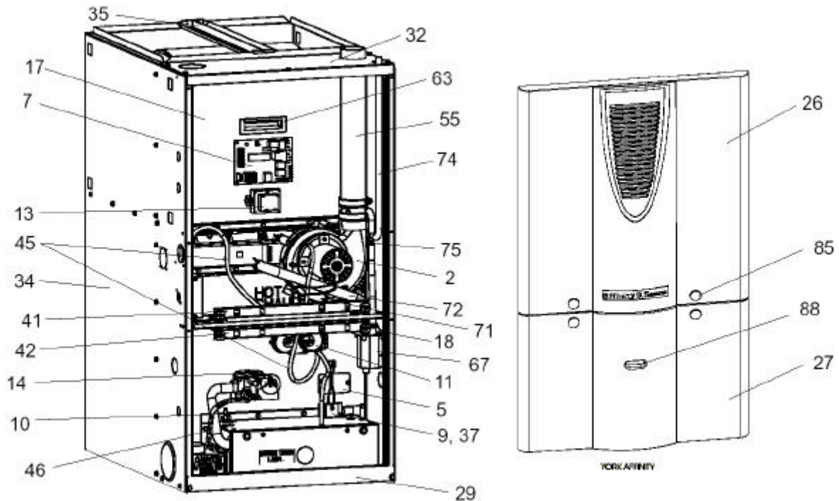
Figure 1: DOWNFLOW/HORIZONTAL NATURAL GAS FURNACES (90%)
