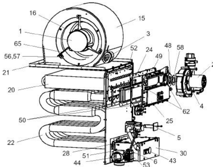
Figure 2: DOWNFLOW/HORIZONTAL NATURAL GAS FURNACES (90%)
