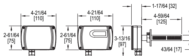
Duct mount
