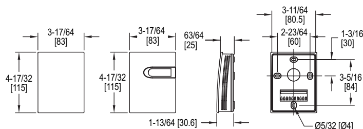
Wall mount
