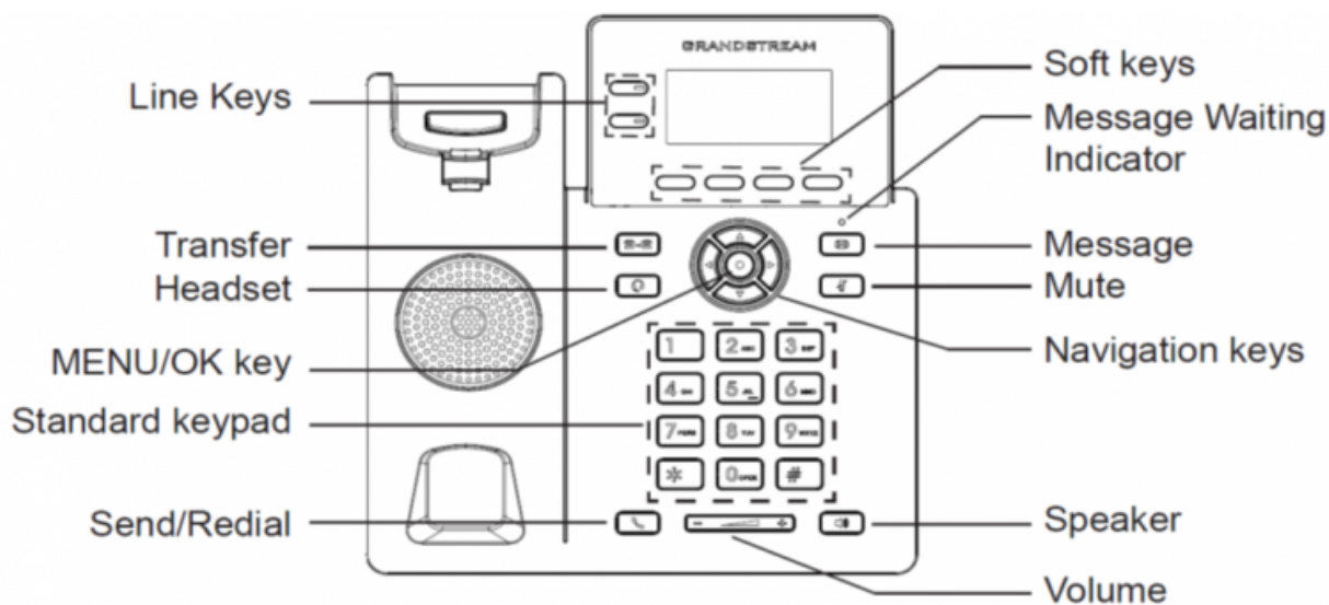
GRP2602 Keyboard
