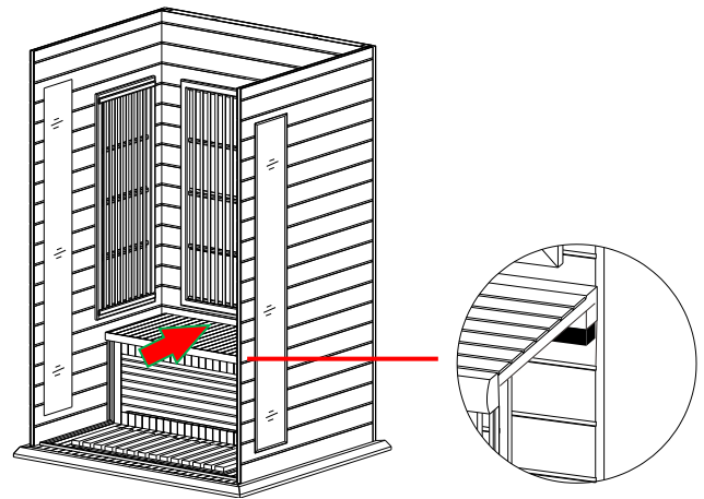
FIG-10 Installing Bench
