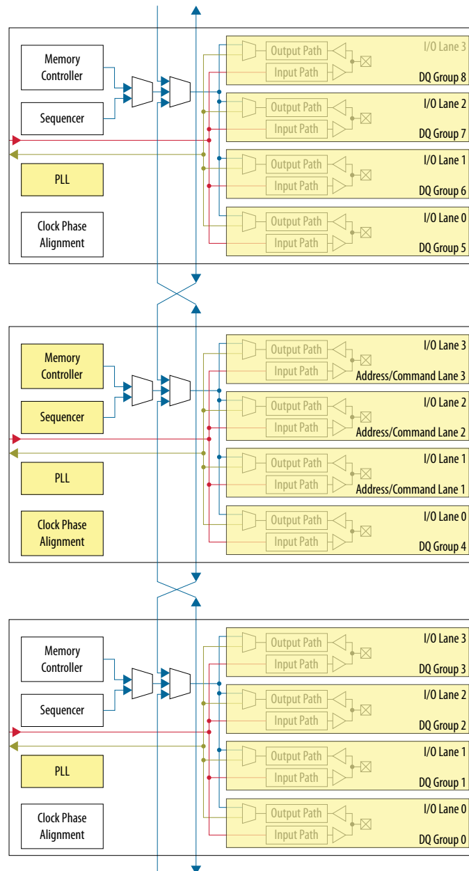
Figure 6. Multi-Bank x72 Interface With Hard Controller
