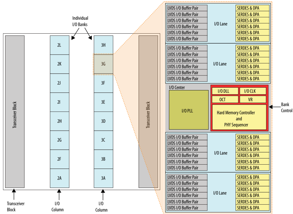
Figure 3. I/O Column
