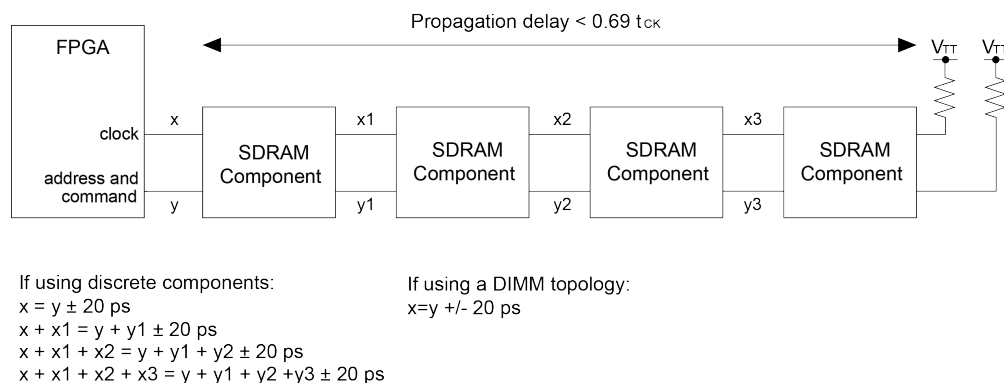
Figure 52. SDRAM Component Address and Command Routing Guidelines
