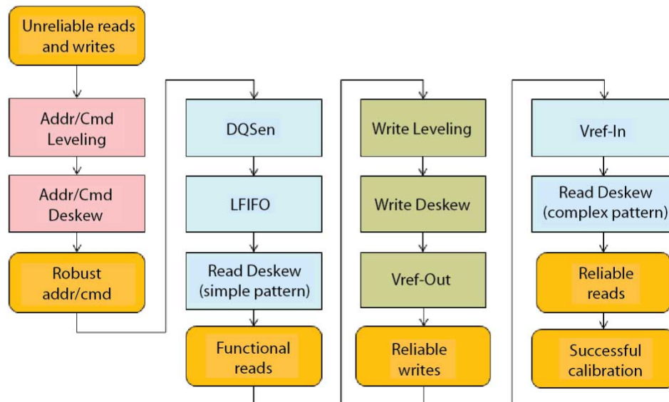
Figure 15. Calibration Flowchart
