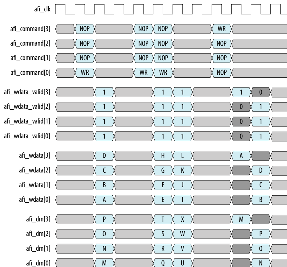
Figure 33. AFI Write Data Quarter-Rate, wlat=1
