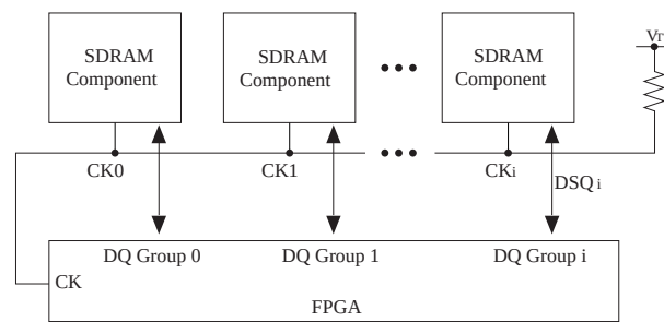
Figure 68. Delaying DQS Signal to Align DQS and Clock
