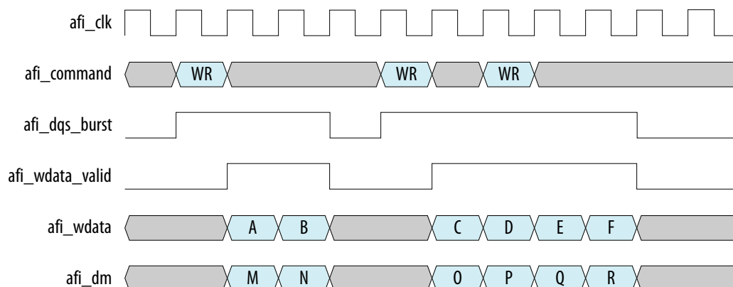
Figure 34. AFI DQS Burst Full-Rate, wlat=1
