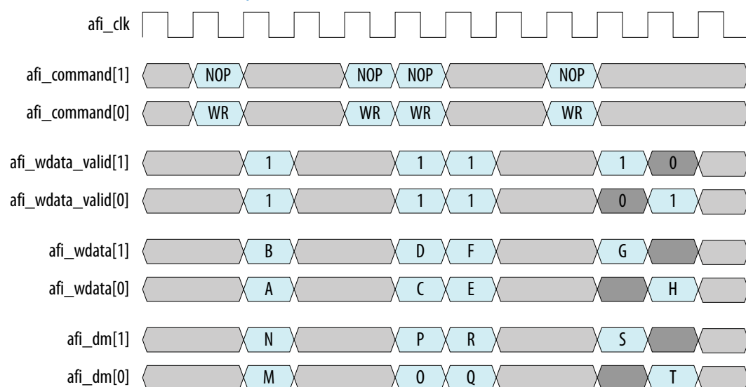
Figure 32. AFI Write Data Half-Rate, wlat=1
