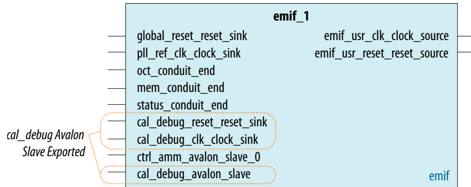
Figure 128. EMIF with EMIF Debug Interface Exported and Daisy-Chain Disabled
