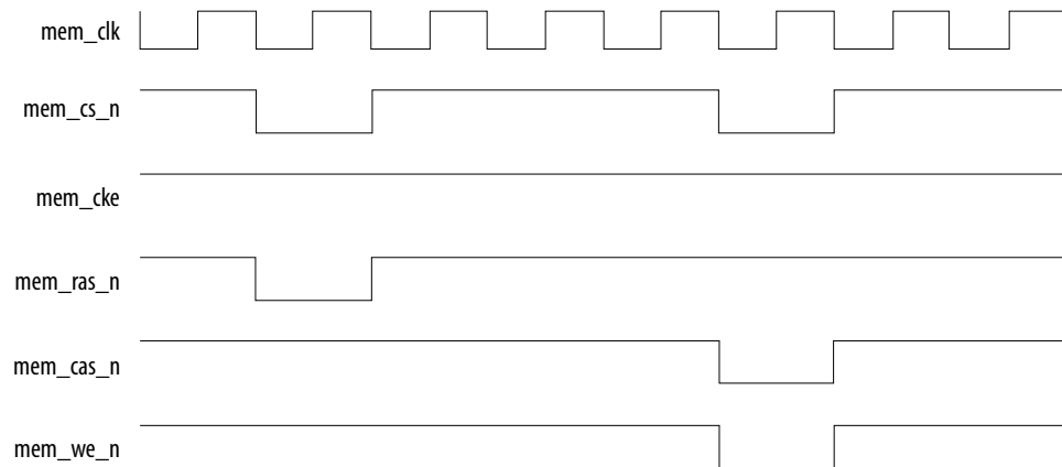
Figure 25. AFI Address and Command Full-Rate
