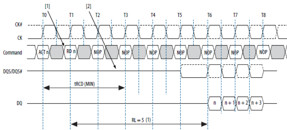
Figure 113. Additive Latency—Read
