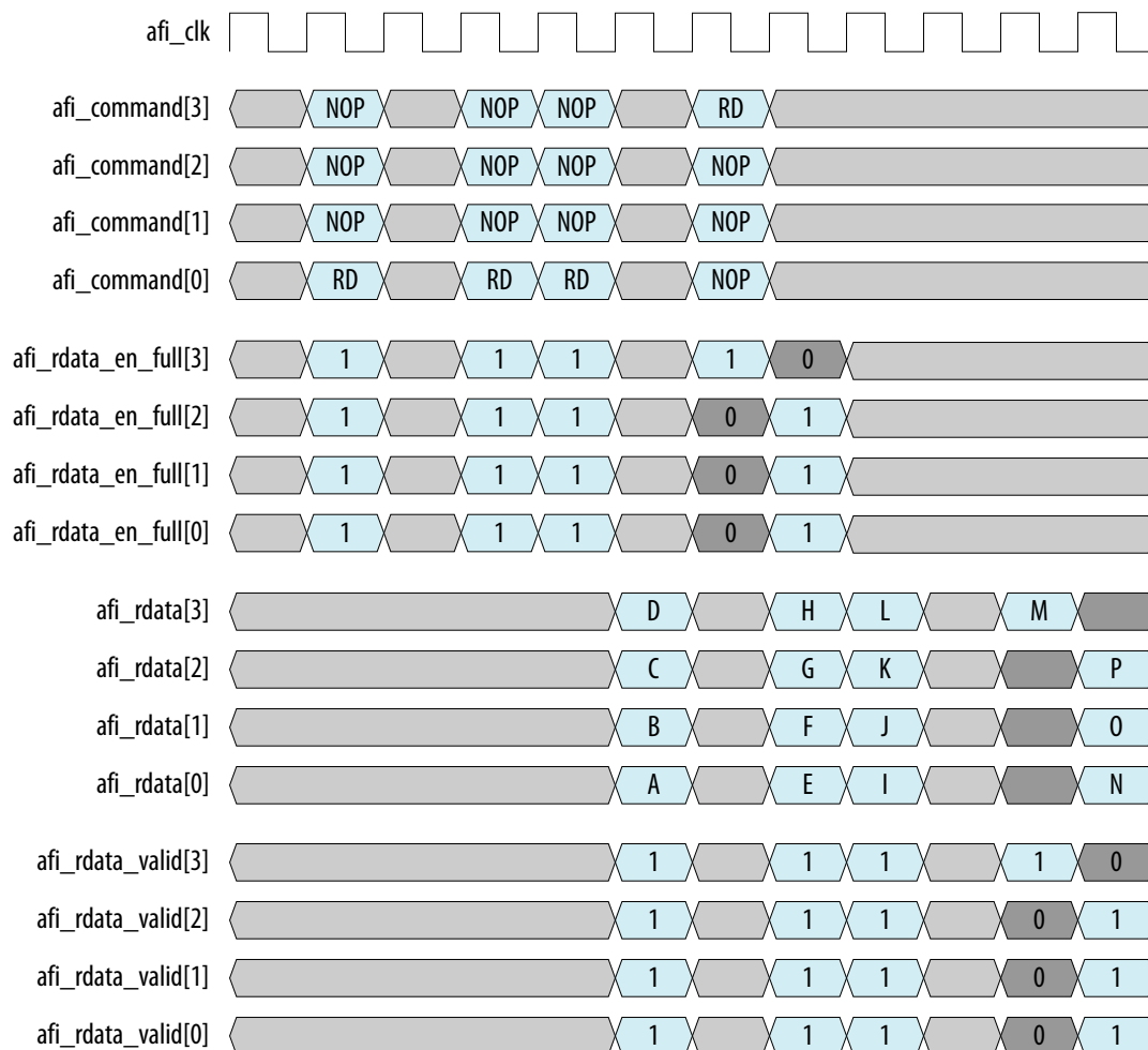
Figure 41. AFI Read Data Quarter-Rate
