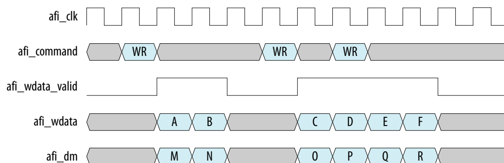
Figure 31. AFI Write Data Full-Rate, wlat=1
