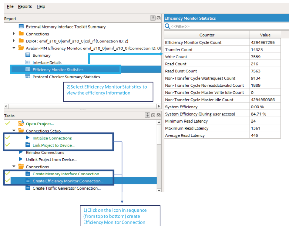
Figure 136. Efficiency Monitor Statistics in the EMIF Toolkit
