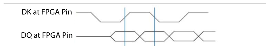
Figure 80. Center-Aligned DQ and DK Relationship During Write
