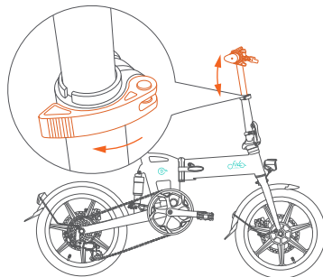
④ Adjust the riser to the suitable height, and close the riser clamp
