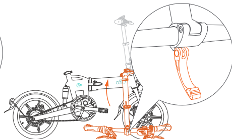
② 2. Open the quick release, adjust the handlebar to the right position. Lift the stem and close the stem clamp to settle it.
