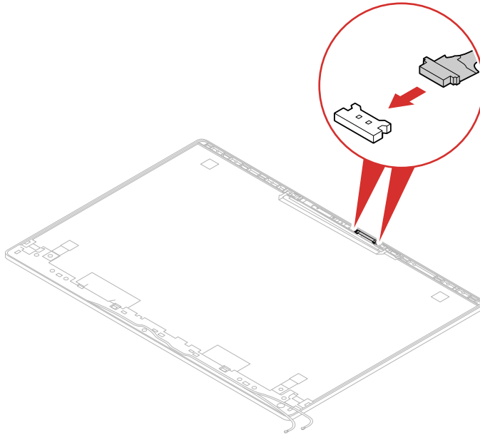
Figure 49. Disconnect the cable between the camera board and microphone board
