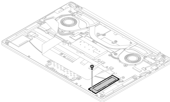
Figure 18. Remove 1 screw
