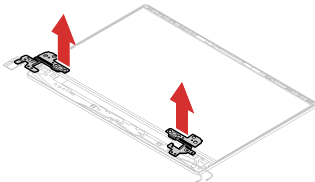
Figure 44. Remove the hinges
