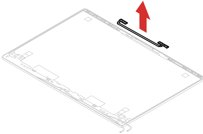
Figure 51. Remove the microphone board
