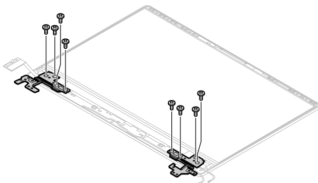
Figure 43. Remove 8 screws
