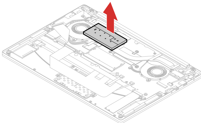
Figure 16. Remove memory module shield
