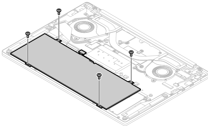
Figure 6. Remove 4 screws
