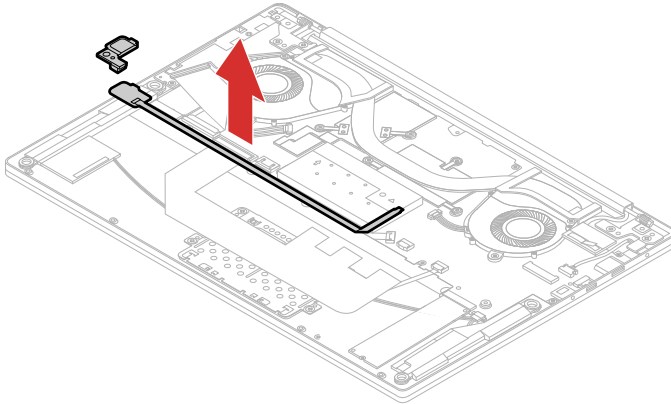
Figure 24. Remove the fingerprint board and its bracket
