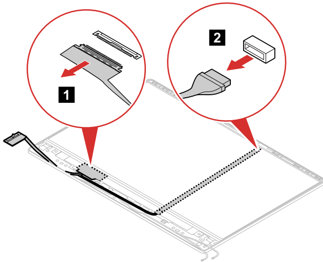
Figure 47. Disconnect 2 cables
