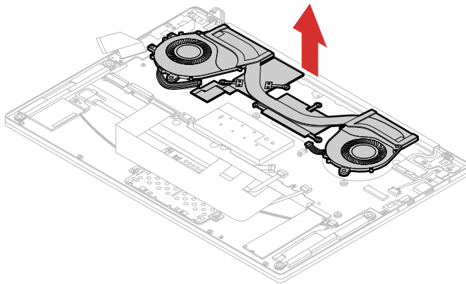
Figure 15. Remove the heat sink and fan assembly
