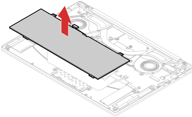
Figure 7. Take out the battery pack
