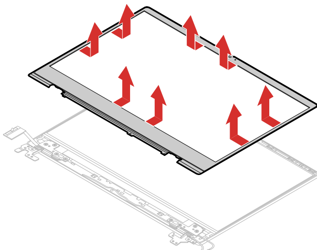
Figure 42. Pull the inner sides of the LCD bezel
