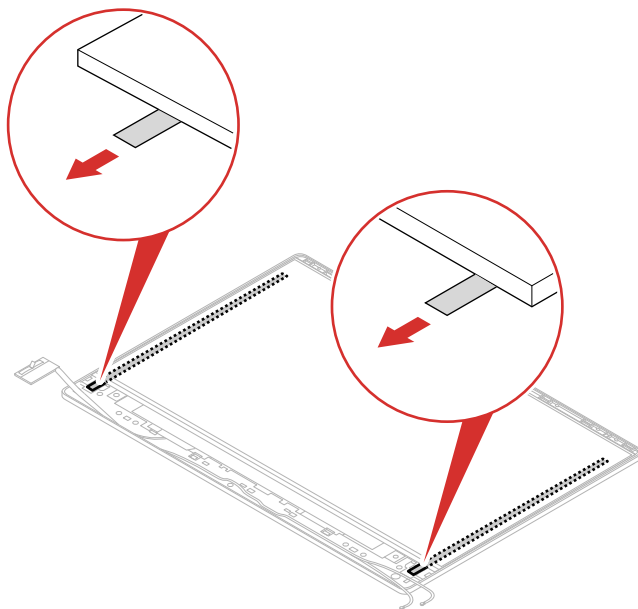
Figure 45. Pull the two tapes
