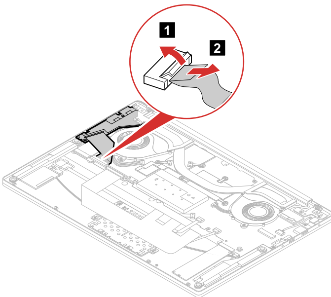
Figure 8. Disconnect the cable
