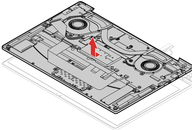
Figure 31. Remove the LCD module
