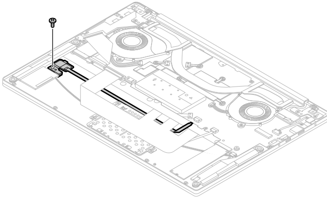
Figure 23. Remove 1 screw
