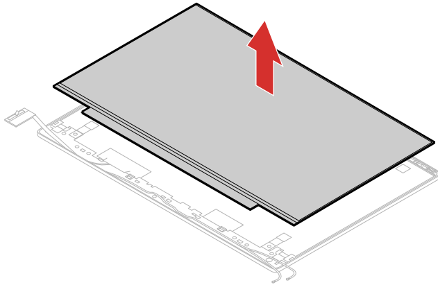
Figure 46. Remove the LCD panel
