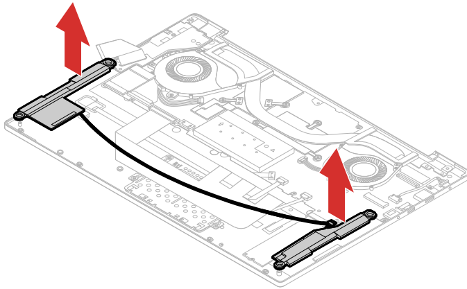
Figure 21. Remove speakers
