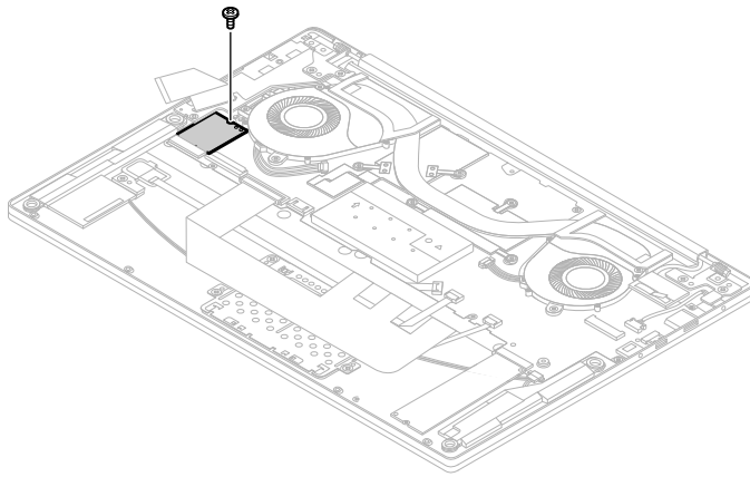
Figure 11. Remove 1 screw
