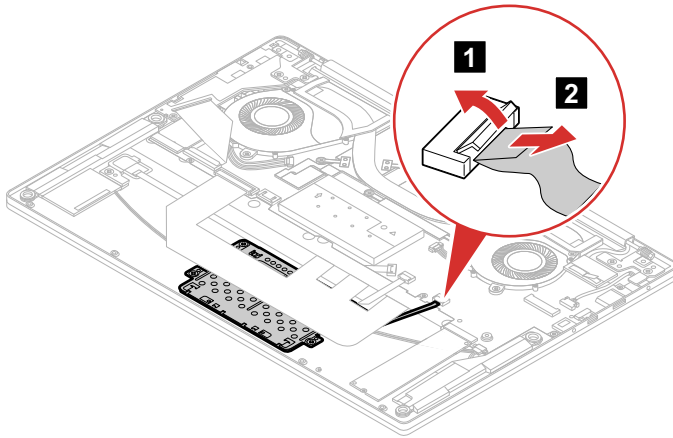
Figure 25. Disconnect the cable
