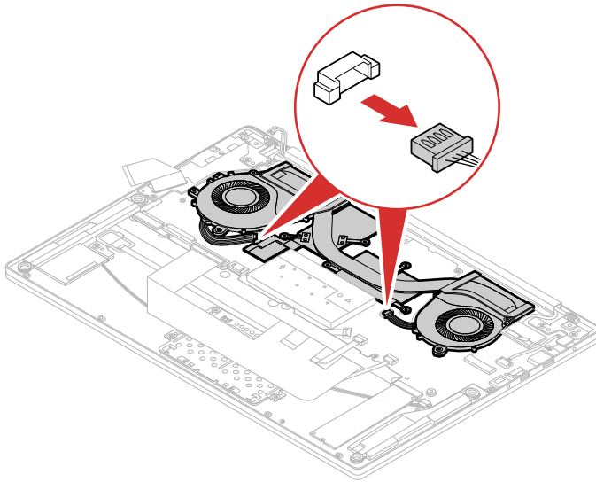
Figure 13. Disconnect 2 cables
