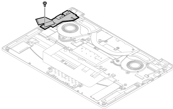
Figure 33. Remove 1 screw
