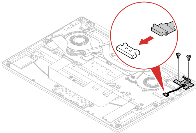
Figure 35. Remove 2 screws and disconnect the cable
