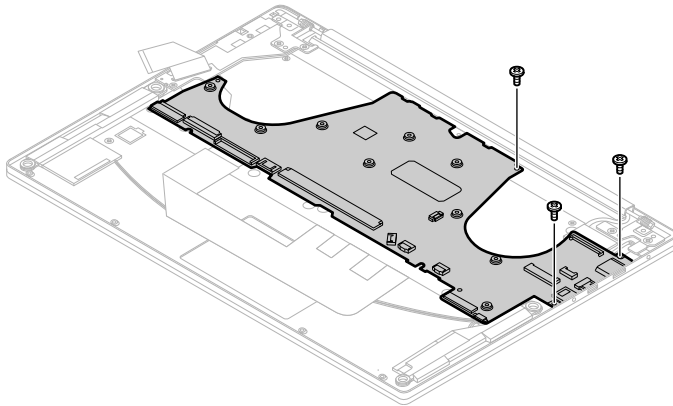
Figure 39. Remove 3 screws
