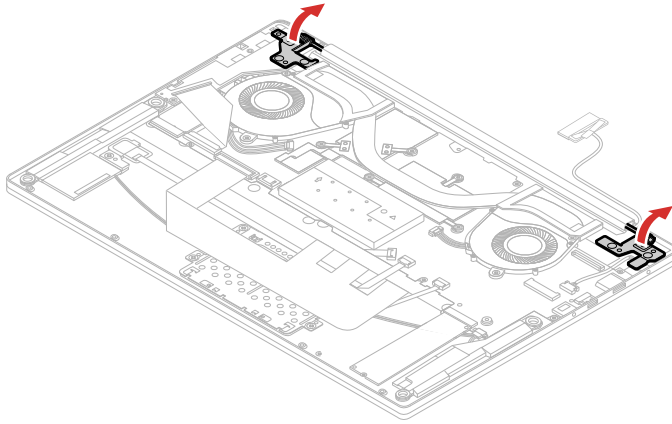
Figure 30. Open the hinges
