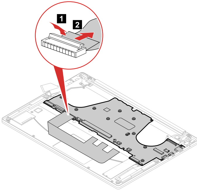
Figure 38. Disconnect the cable
