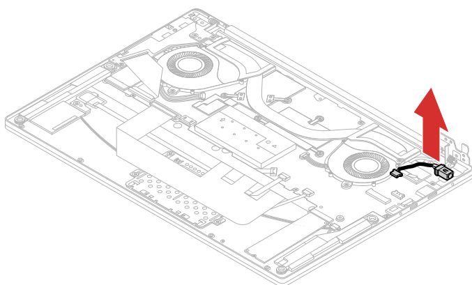
Figure 37. Remove the dc-in cable
