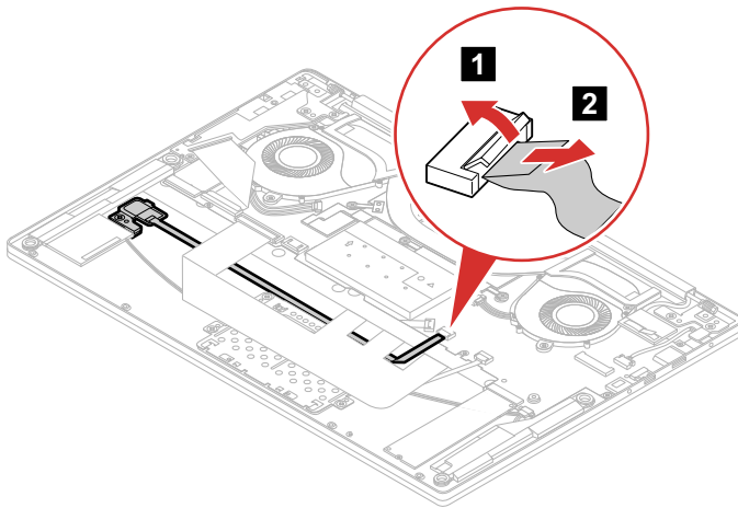
Figure 22. Disconnect the cable
