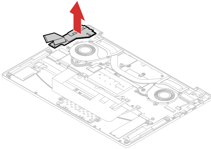
Figure 34. Remove the I/O board
