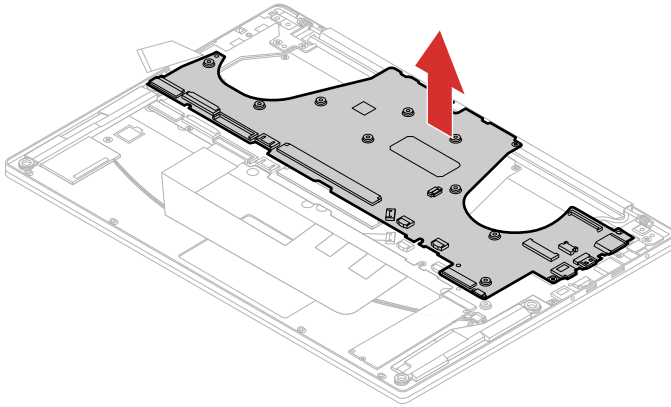
Figure 40. Remove the system board
