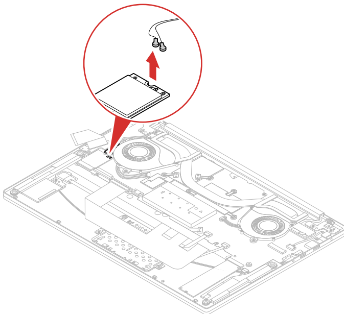
Figure 10. Disconnect antenna cables
