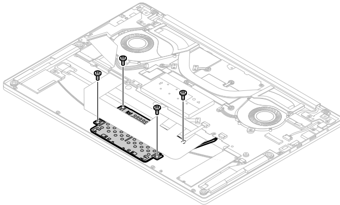
Figure 26. Remove 4 screws
