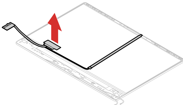
Figure 48. Remove the LCD cable
