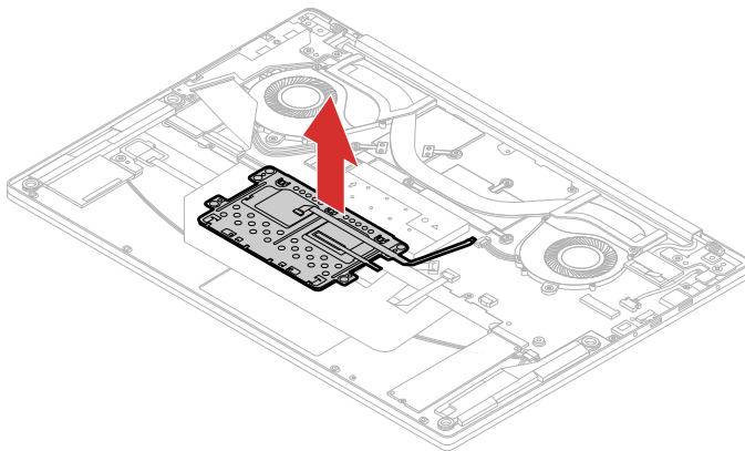
Figure 27. Remove touchpad assembly
