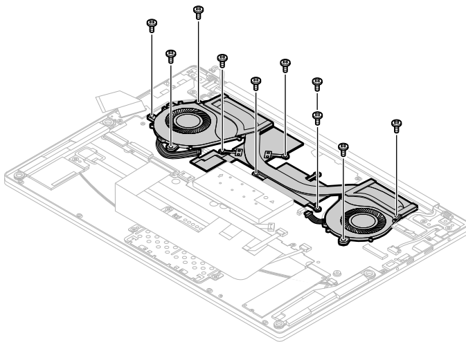
Figure 14. Remove 10 screws
