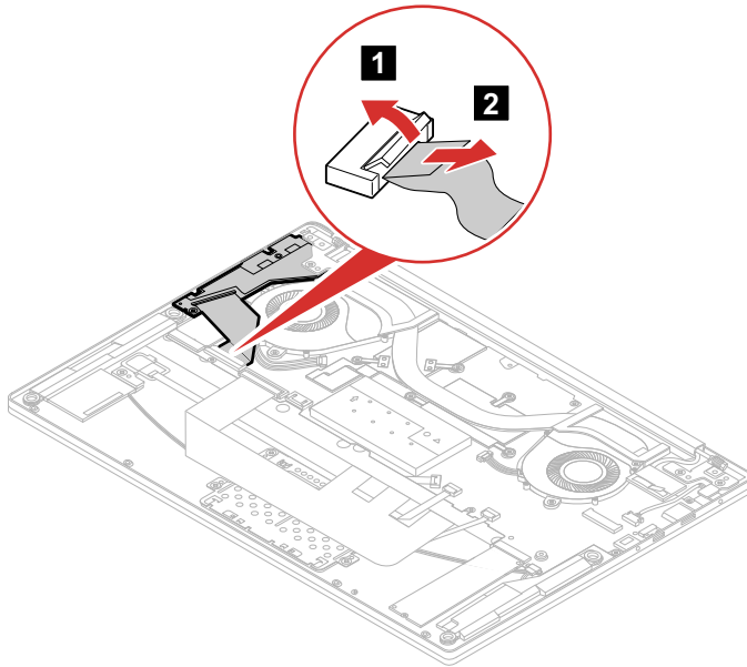
Figure 32. Disconnect the cable
