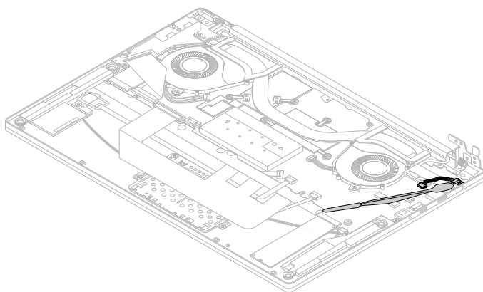
Figure 36. Use a prying tool to detach the dc-in cable from the upper case
