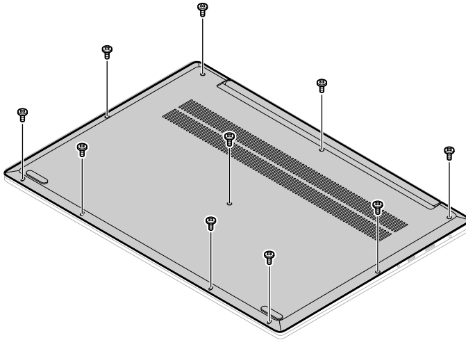
Figure 3. Remove 10 screws
