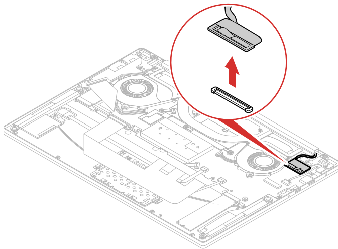
Figure 28. Disconnect the LCD cable
