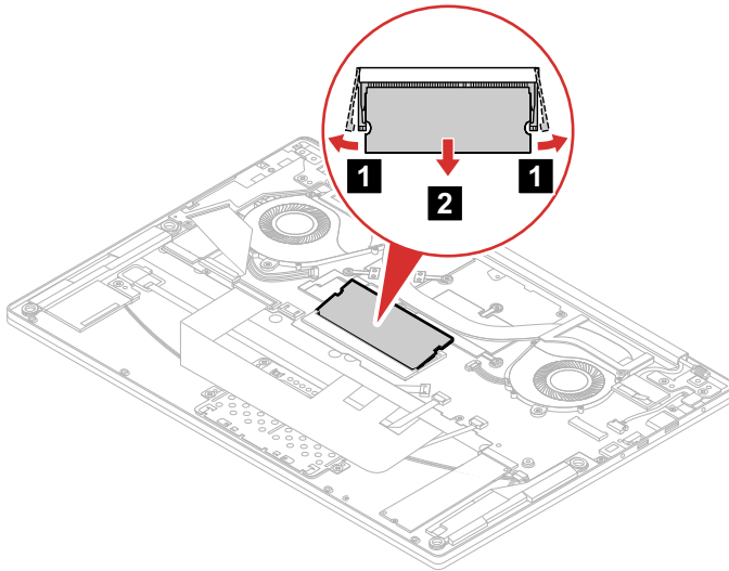
Figure 17. Remove the memory module
