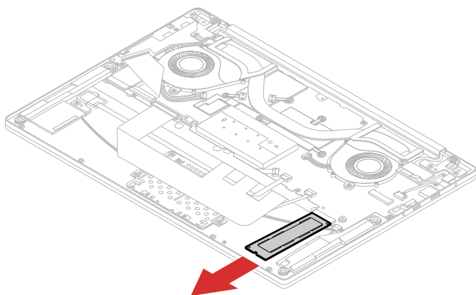
Figure 19. Remove the solid-state drive
