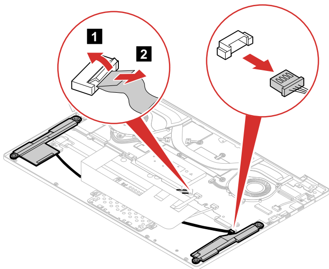
Figure 20. Disconnect 2 cables
