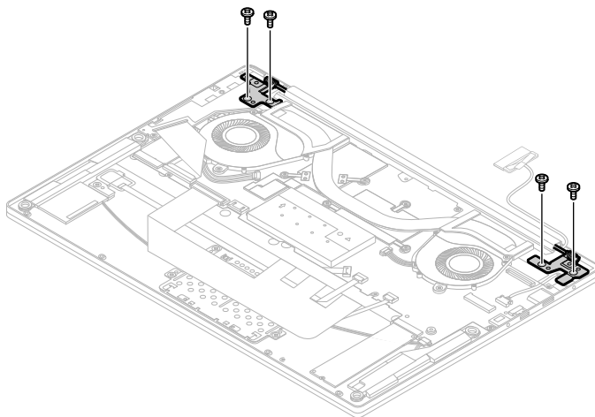
Figure 29. Remove the 4 screws
