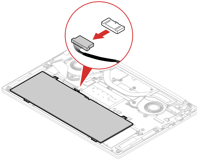
Figure 5. Disconnect the cable
