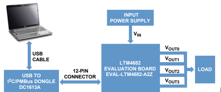
Figure 4. EVAL-LTM4682-A2Z Evaluation Board Setup with a PC
