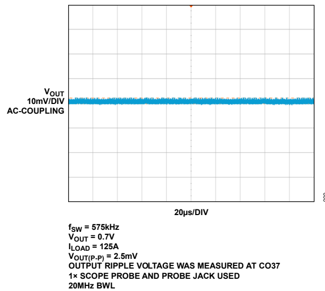
Figure 9. Output Ripple Voltage
