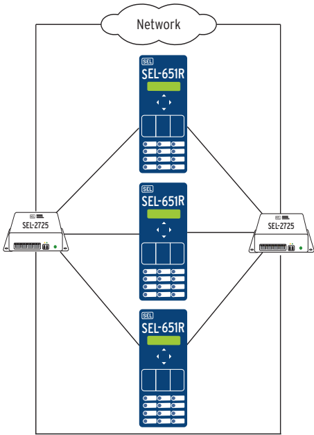
Figure 8 Failover Network Topology
