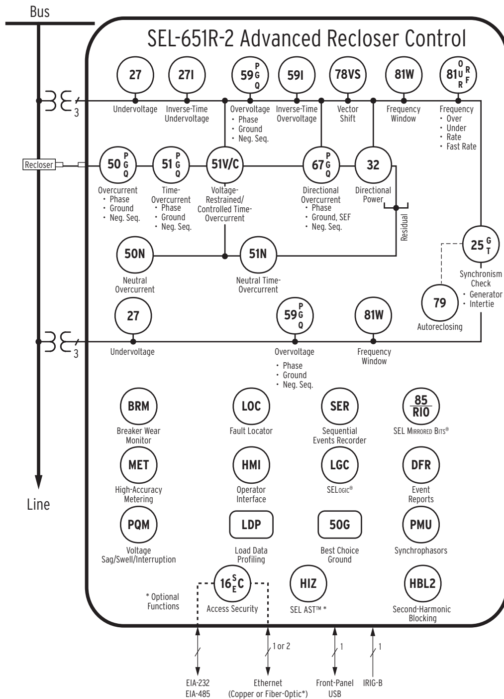
Figure 1 Functional Diagram
