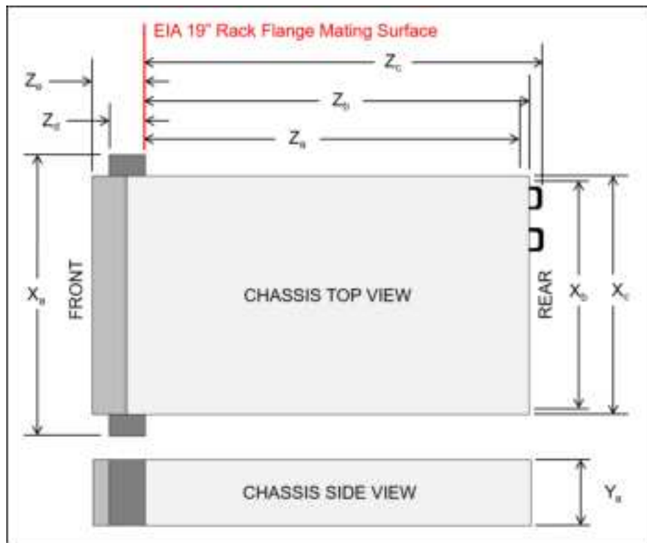
Figure 9. Server dimensions
