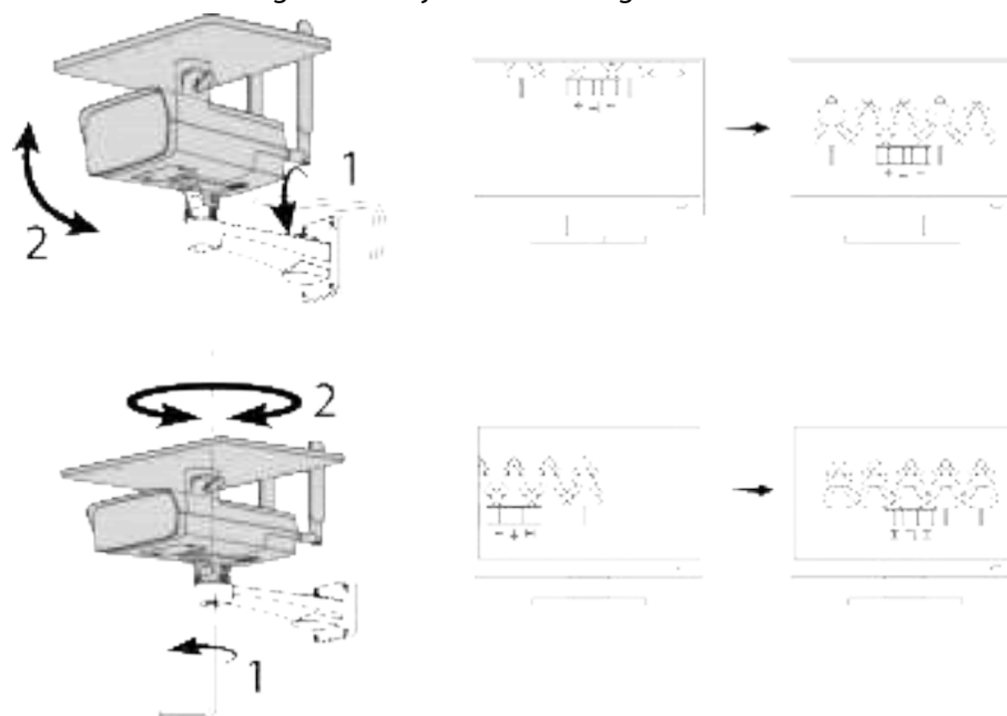
Figure 4-9 Adjust the lens angle
