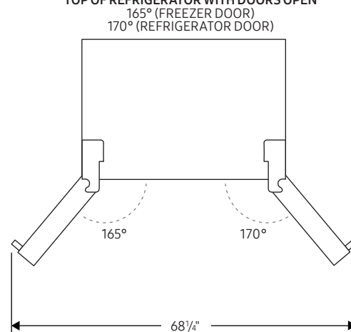
TOP OF REFRIGERATOR WITH DOORS OPEN
