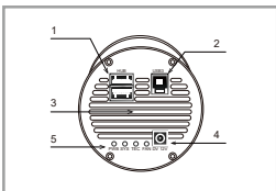
Camera Dimensions and Interface Description
