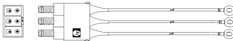
3 Lead HP ECG Lead Wired - 0012-00-0847
