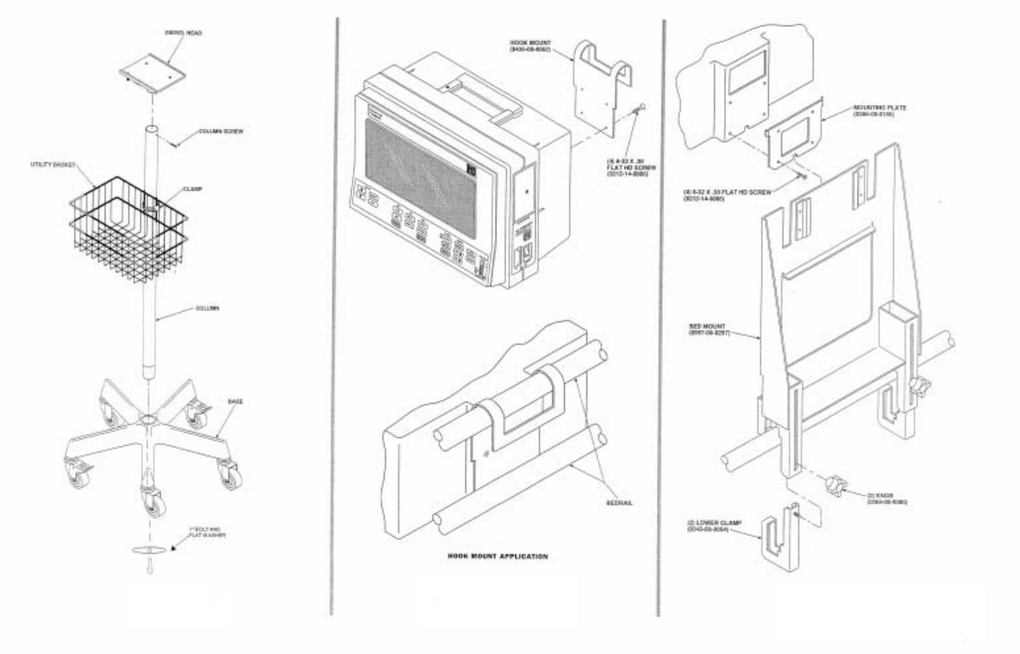
FIGURE 4-1 Rolling Stand 0040-00-0121-02
