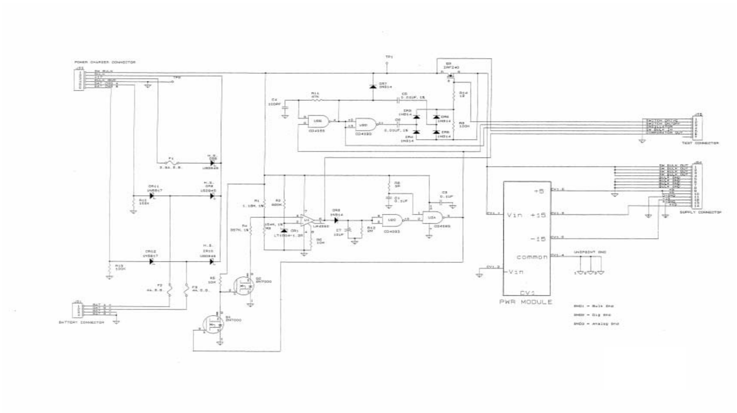
FIGURE 5-10 Line Battery Board 0387-00-0449 0387-00-0621 (5L-CE)
