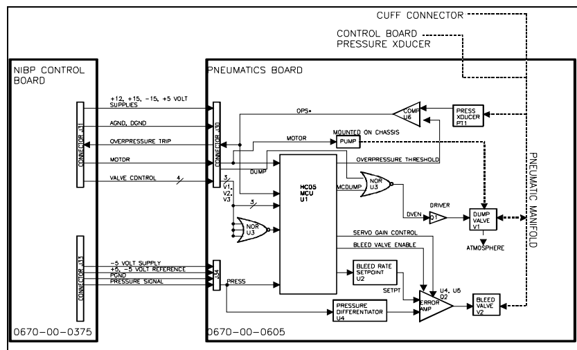
FIGURE 2-27 Linear Bleed Block Diagram
