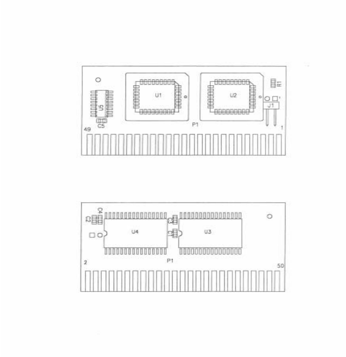
FIGURE 5-49 Datasette Board 0670-00-0574-01 0670-00-0574-03 0670-00-0574-04 0670-00-0574-05
