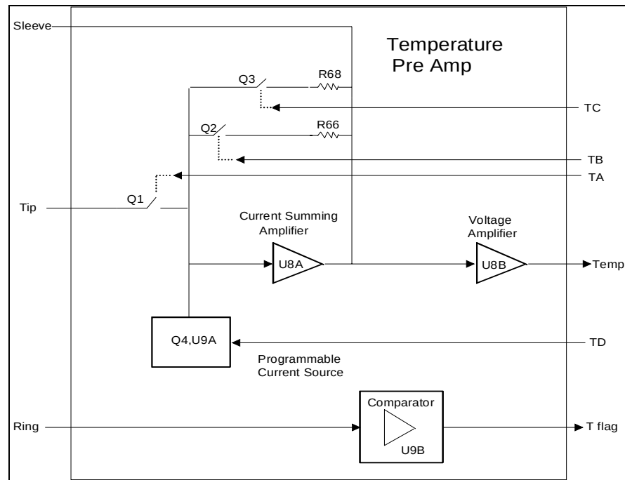
FIGURE 2-10 Temperature PreAmp Block Diagram
