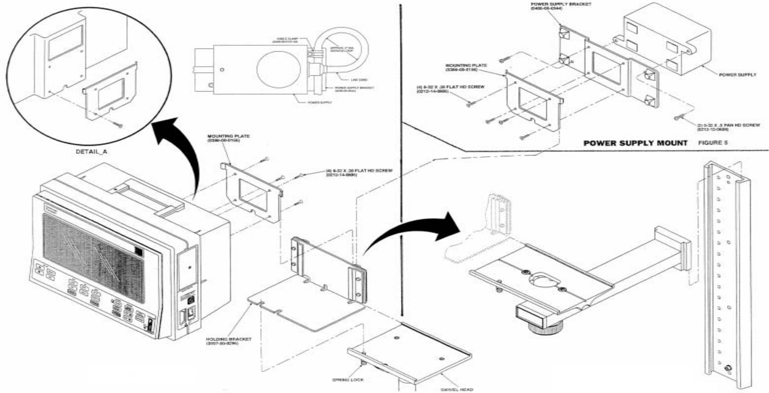
FIGURE 4-4 Passport Mounting
