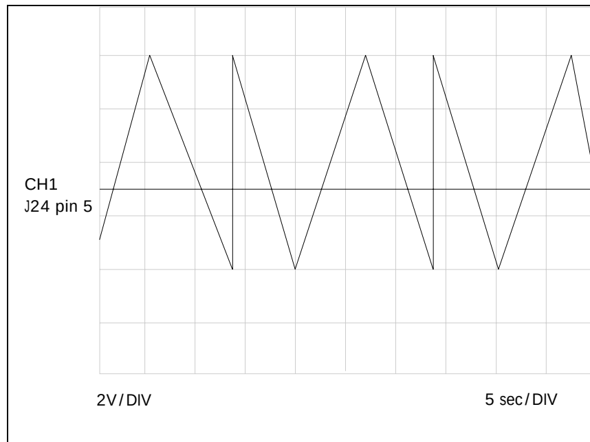
FIGURE 7-10 DAC Waveform
