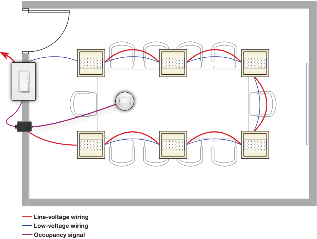
With power pack (DVTV Only)
