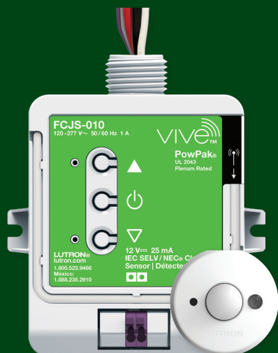
PowPak wireless fixture controller and PowPak fixture sensor
