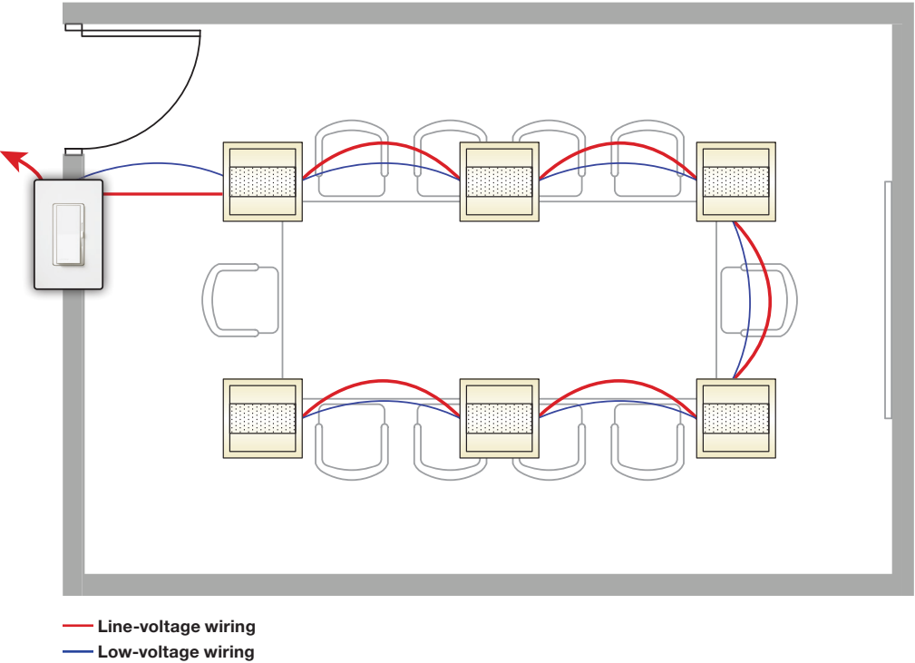
Without power pack (DVSTV Only)
