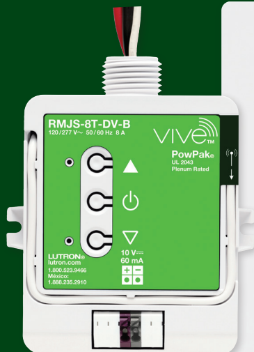
PowPak dimming module with 0–10V control
