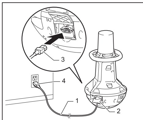
► 1. Power cord 2. Socket cover (AC inlet) 3. Plug (for the appliance) 4. Plug (for an outlet)
