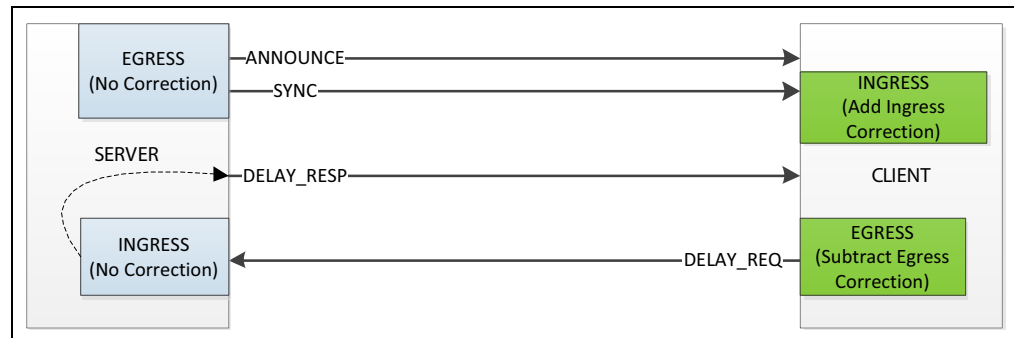
FIGURE 6-2: Overview of Delay Asymmetry in Client-Server Configuration.
