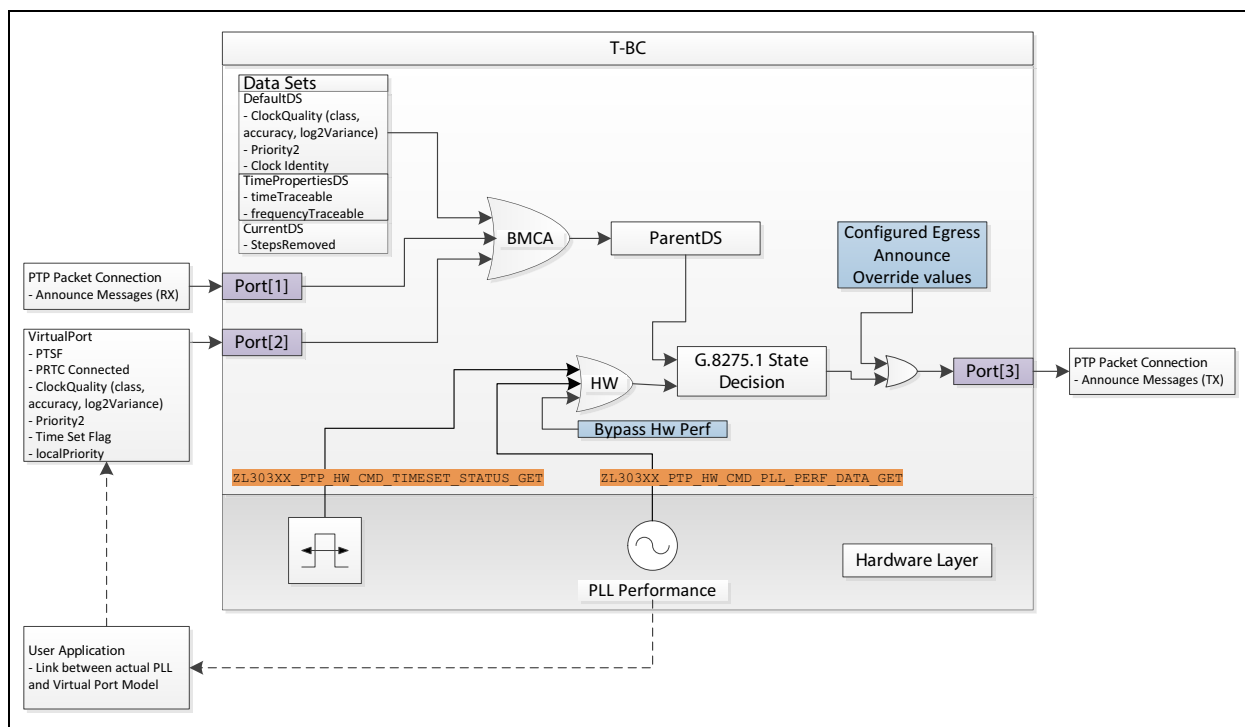
FIGURE A-1: General G.8275.1 System Operation.
