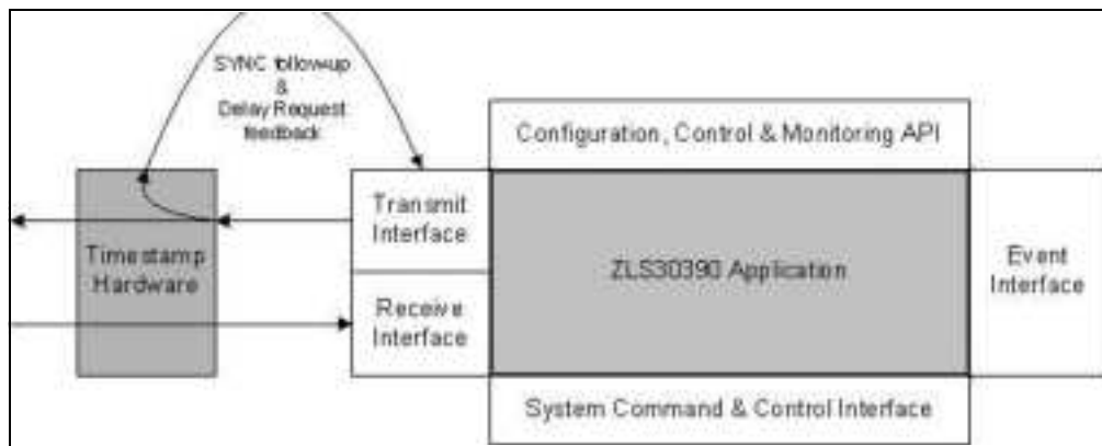
FIGURE 10-1: PTP Overview.
