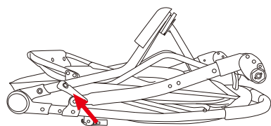
Folding hook
