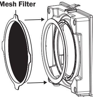
Outer Nylon Mesh Filter
