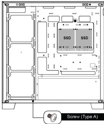
SSD Drive Installation
