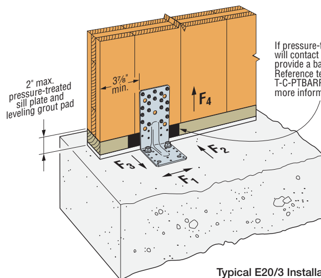
Typical E20/3 Installation at CLT Wall on Concrete Curb or Grout Pad
