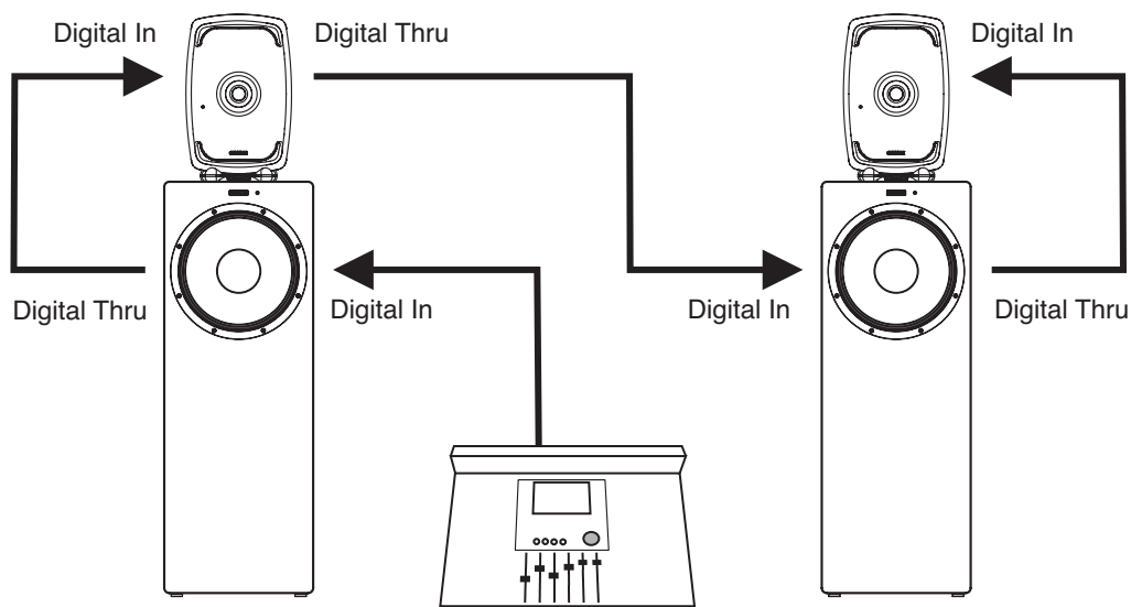
Figure 10. Cabling for AES/EBU digital audio
