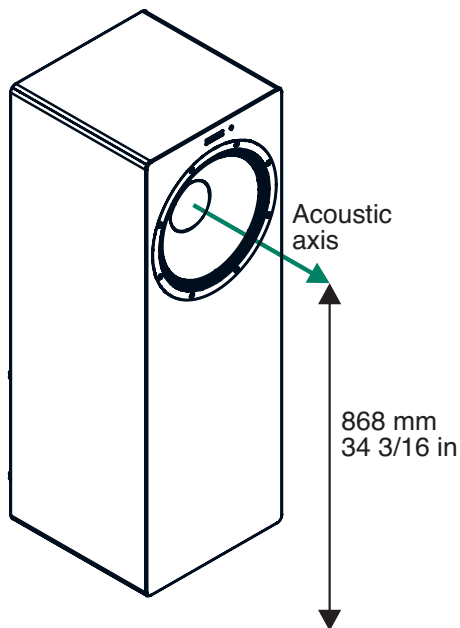
Figure 5. Location and orientation of the acoustic axis
