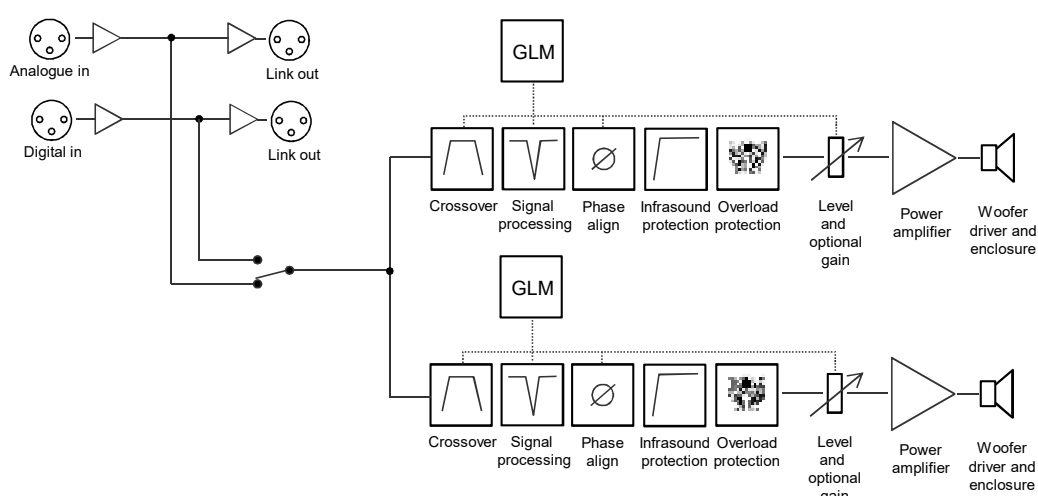
Figure 4. Functional block diagram of the W371A
