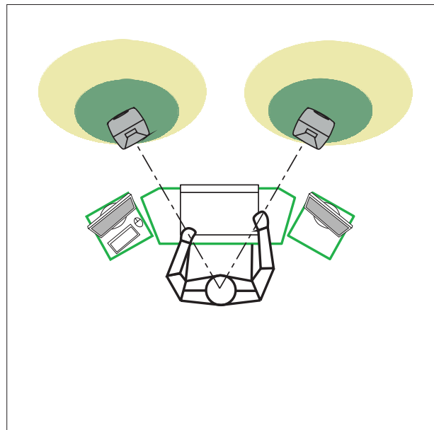
Figure 6. Guidelines for placement of the W371A relative to the monitors. Green area is recommended, yellow acceptable
