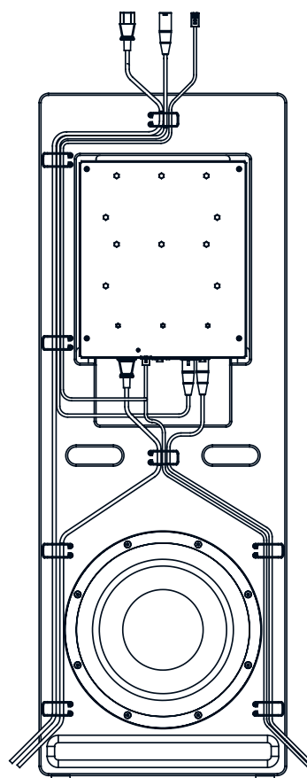
Figure 7. Examples of routing cables using the provided cable management clips. Do not run cables over the woofer transducer.
