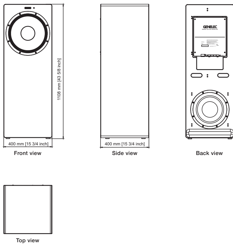
Figure 16. Dimensions of the W371
